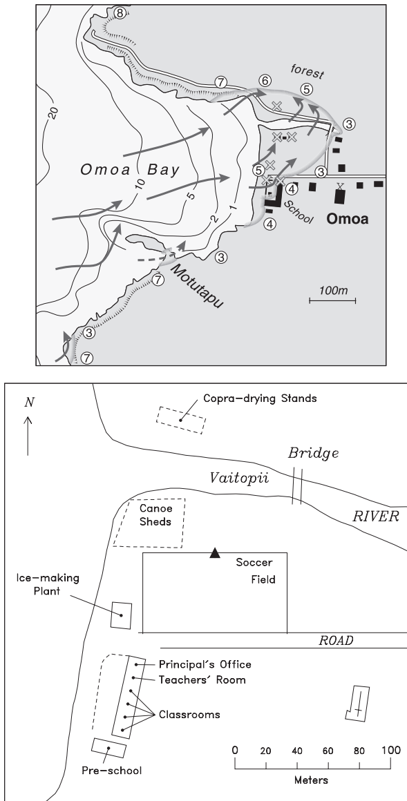
FIG. 2. – Top : Map of inundation around Omoa Bay. Circled numbers are runup amplitudes in meters, the thick line is the limit of penetration of the waves, and the arrows sketch the deflection of the waves by Motutapu. Crosses identify damaged or destroyed structures. Bathymetric contours in Omoa Bay are in meters. Bottom : Close-up map of the beach front of the village of Omoa. Dashed lines identify structures destroyed beyond repair. The school complex is detailed at lower left, including the destroyed wall around the school yard (dashed). The solid triangle shows the location where the compressor unit from the ice-making plant was deposited.
