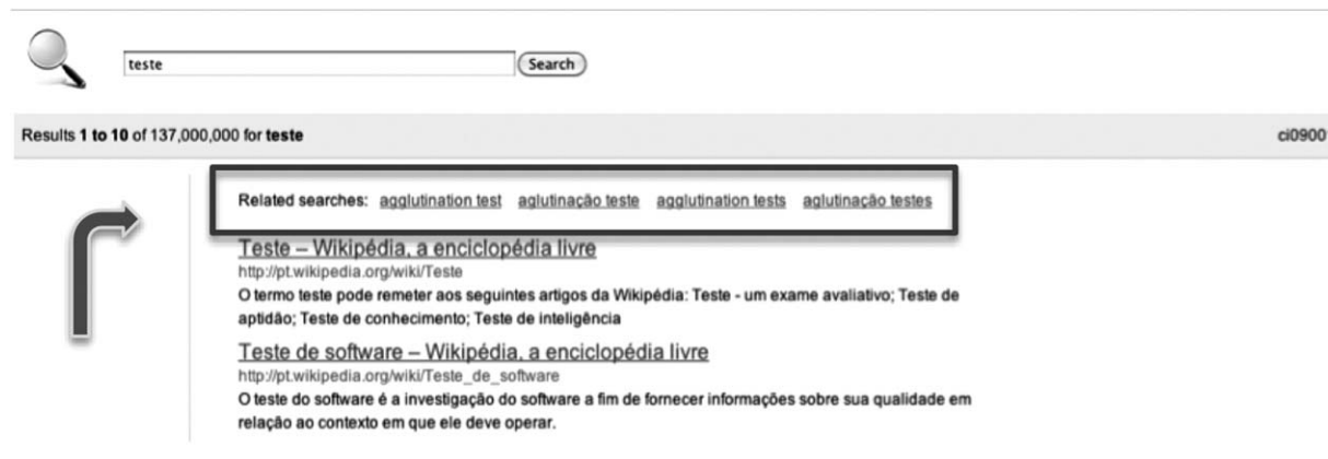
FIG. 2. Results page for the system presenting query suggestions.
