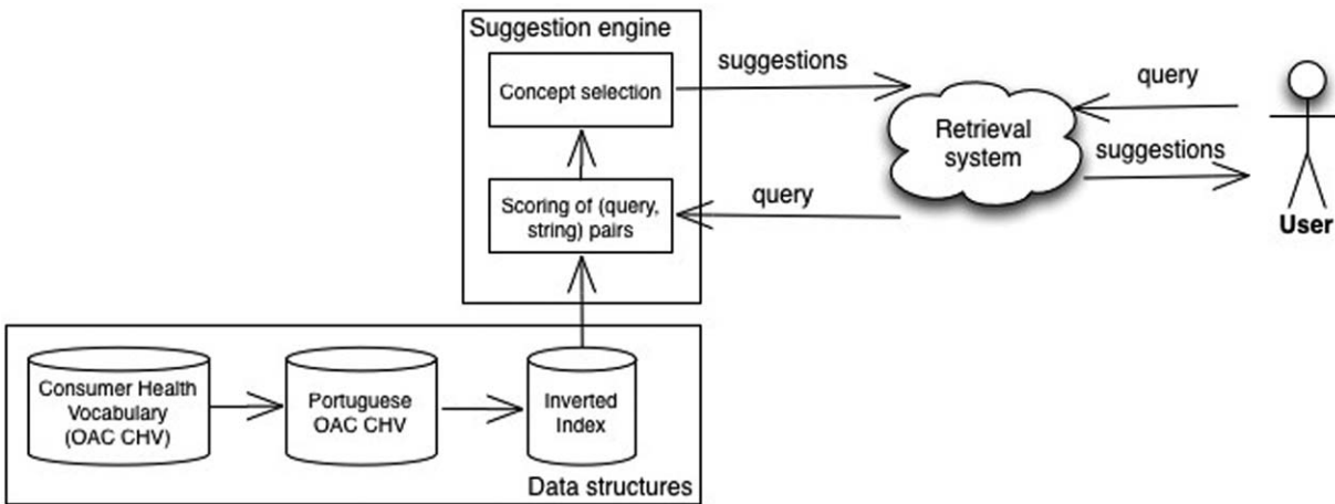
FIG. 1. Architecture of the suggestion tool.
