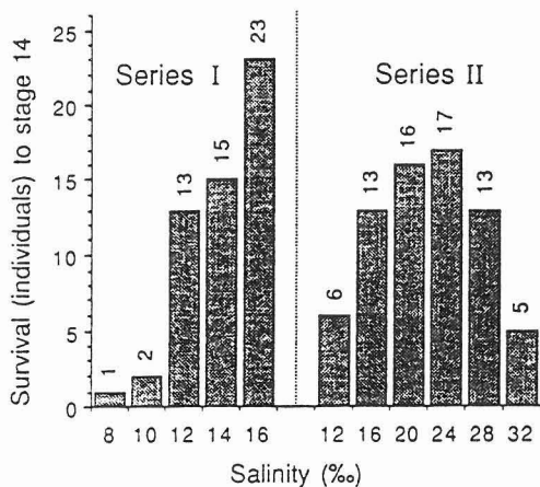
Figure 10. — Number of Macrobrachium collehovenii larvae surviving to stage XIV (reared individually with initial n = 50 ) in different salinities.
