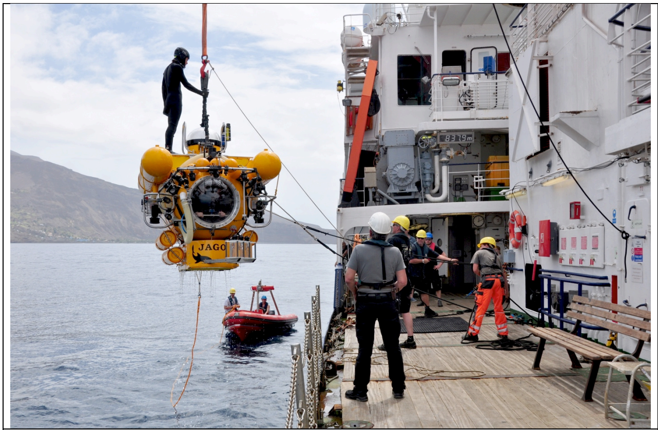
GEOMAR's research submersible JAGO recovered after a dive off Santo Antao
