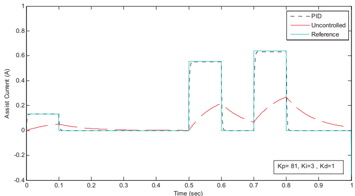
Fig 5: Controller Performance between PID and Uncontrolled System
