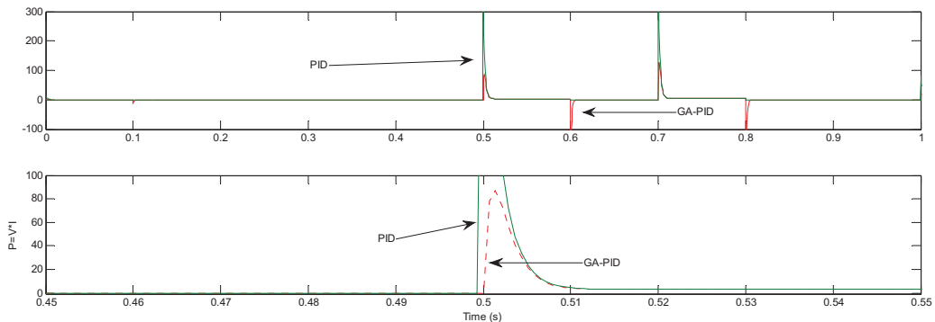
Fig 8: Power Consumption of PID and GA-PID
