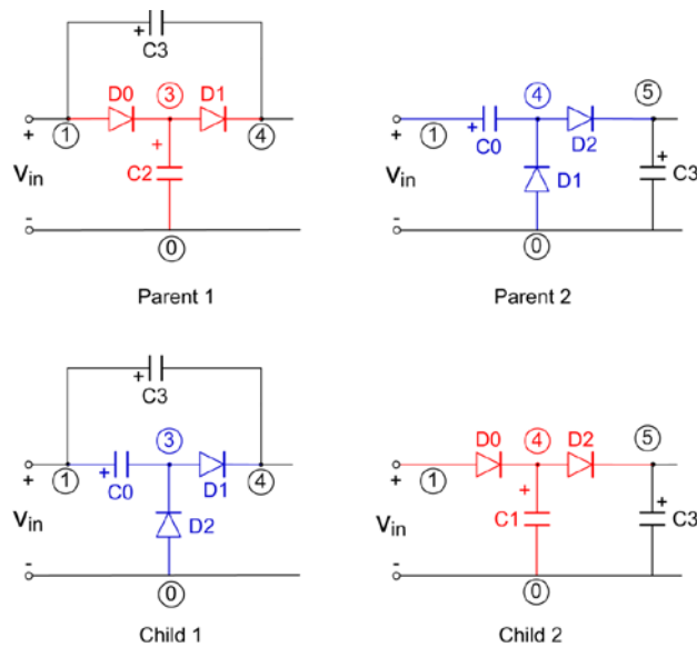
Fig. 3. Example of crossover between two parent circuits.
