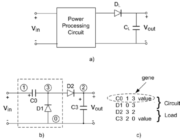
Fig. 1. Structure of the test circuit a) Test circuit b) Example of circuit with named devices and nodes c) Circuit representation.
