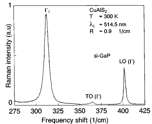
FIG. 8. Room temperature Raman spectrum of \text{CuAlS}_2 obtained in the backscattering configuration from (112) plane for parallel polarization of the incident and scattered light and of \text{si-GaP} obtained also in the backscattering configuration from (111) plane for identical experimental conditions including the same incident power of 2 mW and detection intensity scale. Notice the large absolute scattering intensity of \Gamma_1 phonon mode at 314 \text{ cm}^{-1} in comparison with \text{LO}(\Gamma) phonon mode at 402.3 \text{ cm}^{-1} of \text{Si-GaP} .
