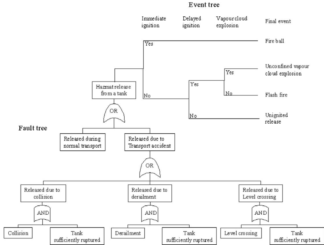
Fig. 5. A fault tree in conjunction with an event tree for hazmat release (adapted from Alp, 1995).
