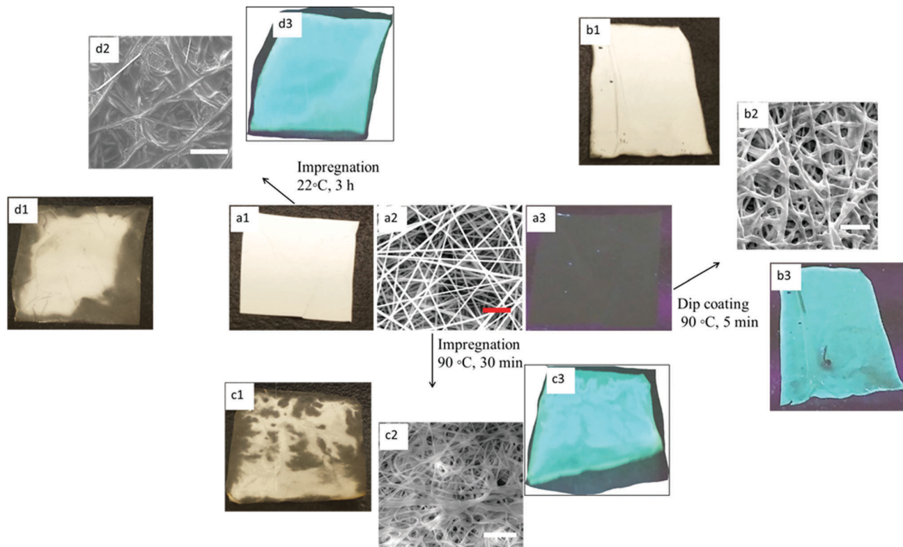
Fig. 3 (a1) Electrospun Nylon 6,6-NF under visible light. (a2) Representative SEM image of the Nylon 6,6-NF (scale bar = 1 \mu\text{m} ). (a3) Nylon 6,6-NF under UV light. (b1) Si QD-90-decorated Nylon 6,6-NF by dip coating under visible light. (b2) Representative SEM image of the Si QD-90-decorated Nylon 6,6-NF by dip coating (scale bar = 1 \mu\text{m} ). (b3) Dip-coated Si QD-90-decorated Nylon 6,6-NF under UV light. (c1) Si QD-90-decorated Nylon 6,6-NF by the impregnation method and at 90 ^{\circ}\text{C} , 30 min drying, under visible light. (c2) Representative SEM image of the Si QD-90-decorated Nylon 6,6-NF by the impregnation method and at 90 ^{\circ}\text{C} , 30 min drying (scale bar = 2 \mu\text{m} ). (c3) Impregnation method, Si QD-90-decorated and at 90 ^{\circ}\text{C} , 30 min dried Nylon 6,6-NF under UV light. (d1) Impregnation method, Si QD-90-decorated air (22 ^{\circ}\text{C} ) 3 h dried Nylon 6,6-NF under visible light. (d2) Representative SEM image of the impregnation method, Si QD-90-decorated Nylon 6,6-NF (scale bar = 2 \mu\text{m} ). (d3) Impregnation method, Si QD-90-decorated and air (22 ^{\circ}\text{C} ) 3 h dried Nylon 6,6-NF under UV light.
