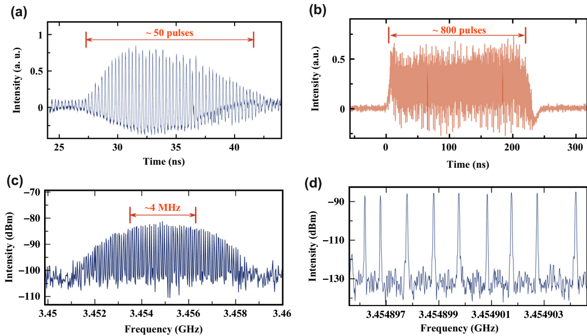
Fig. 3. (a) Measured output pulse train for the 15 ns-long burst after dechirping. (b) 230 ns-long burst train containing approximately 800 pulses. (c) Measured RF spectra of the amplified burst train over a span of 10 MHz, centered at 3.455 GHz, the width of which is determined by the burst duration of 230 ns. (d) Close-up of the RF spectrum in (c) showing densely spaced comb lines of 1-kHz spacing over a span of 10 kHz.
