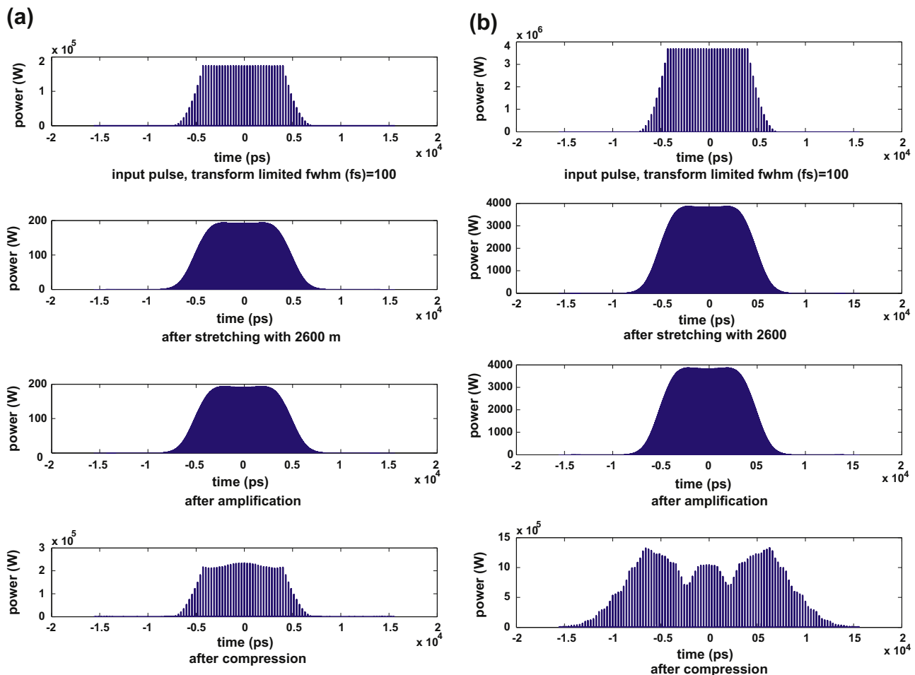
Fig. 5. Simulation results for 50-pulse bursts with intra-burst pulse repetition period of 285 ps, with the pulses being stretched to 2 ns, then traversing a nonlinear optical segment, before being dechirped, for (a) low nonlinear phase shift in the amplifier, and (b) 20 times higher nonlinear phase shift in the amplifier.
