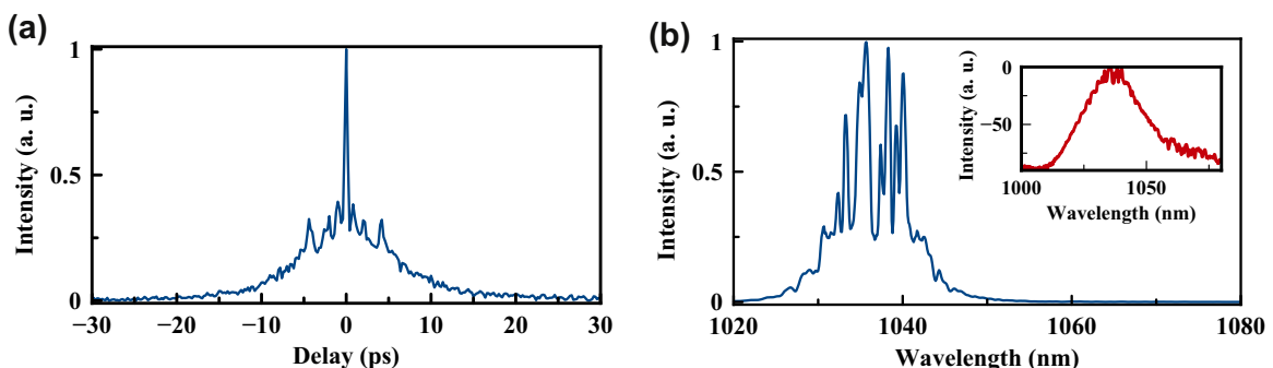
Fig. 4. (a) Measured autocorrelation for a burst energy of 200 \mu\text{J} , burst duration of 15-ns, and containing approximately 50 pulses per burst. (b) Measured output optical spectrum for the same conditions as in (a). Inset: semi-log version.
