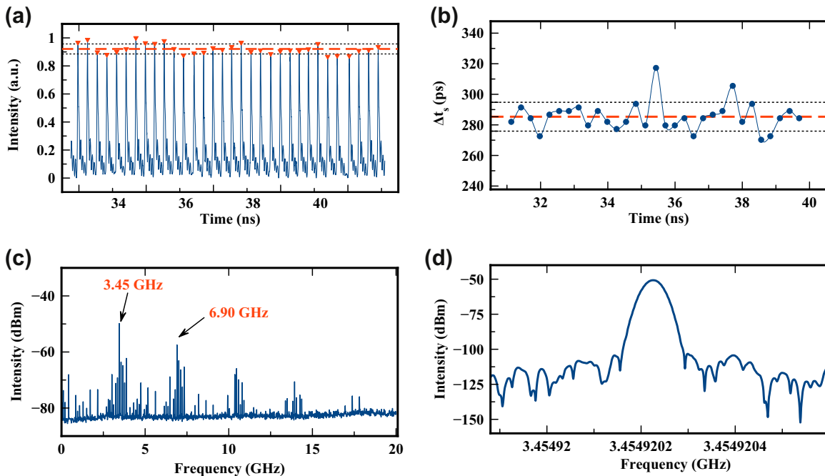
Fig. 2. (a) Temporal profile of 3.5-GHz pulse train measured after the repetition rate multiplier. (b) Measured deviation from average pulse separation time. Dashed (red) line indicates average and dotted (black) line indicates one standard deviation. (c) Measured RF spectrum with 20 GHz span and 100 kHz resolution. (d) Measured close-up RF spectrum with 10 kHz span and 20 Hz resolution. (For interpretation of the references to color in this figure caption, the reader is referred to the web version of this paper.)
