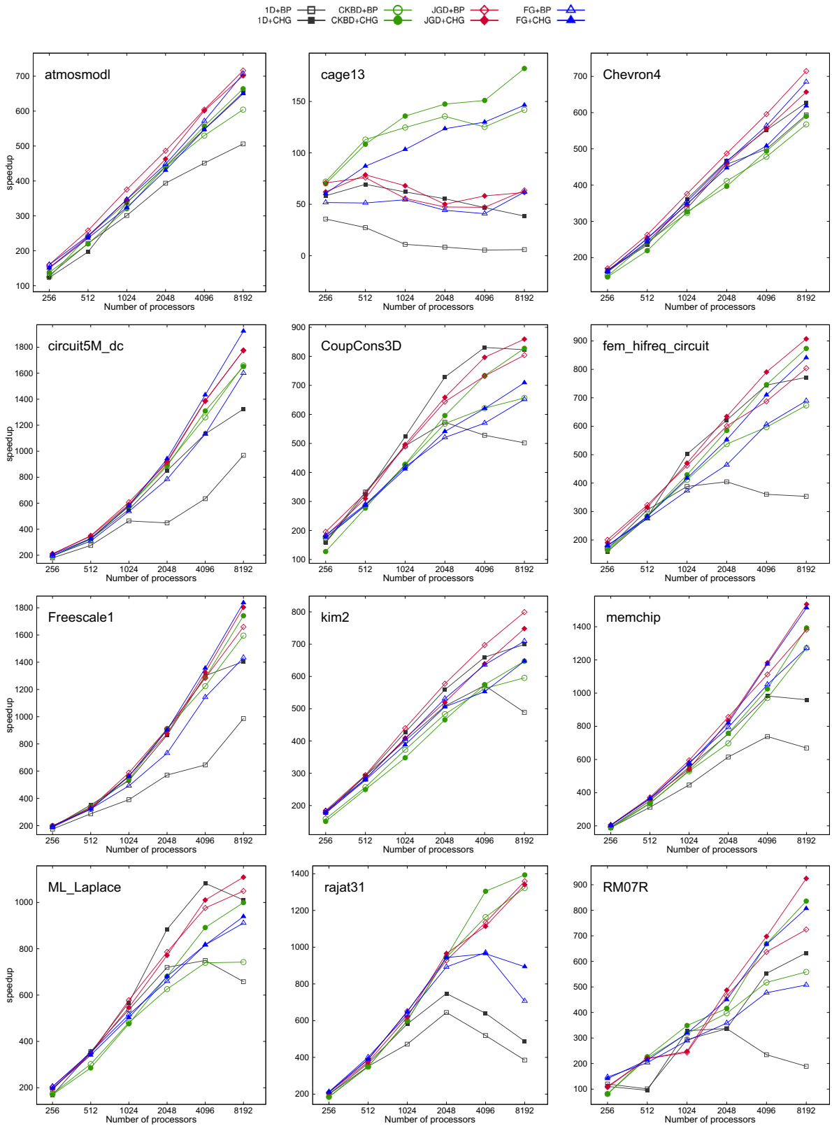
Fig. 9. Speedup curves.
