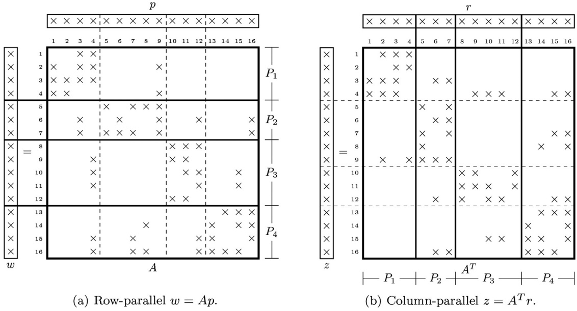
Fig. B.10. Row-parallel matrix-vector and column-parallel matrix-transpose-vector multiplication.
