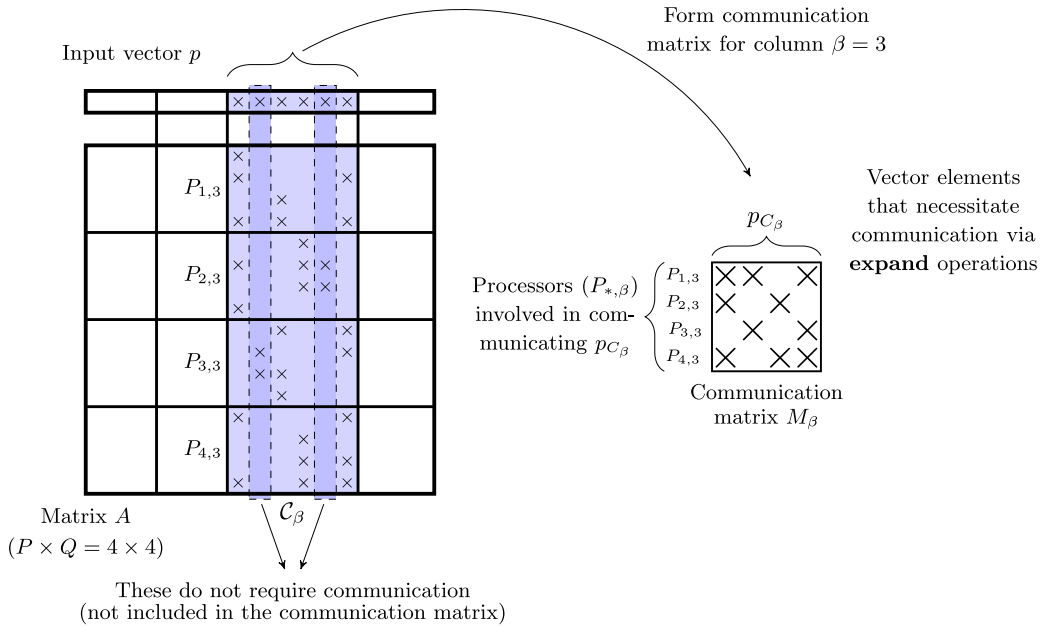
Fig. 2. Formation of the communication matrix for the third column of the processor mesh ( \beta = 3 ) to summarize expand operations in the pre-communication stage.
