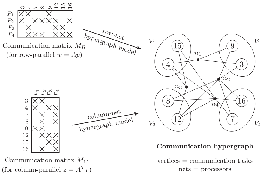
Fig. D11. Formation of the communication hypergraph from a communication matrix, and a four-way partition on this hypergraph. Matrices M_R and M_C summarize the communication requirements of w = Ap and z = A^T r operations illustrated in Fig. B.10.
