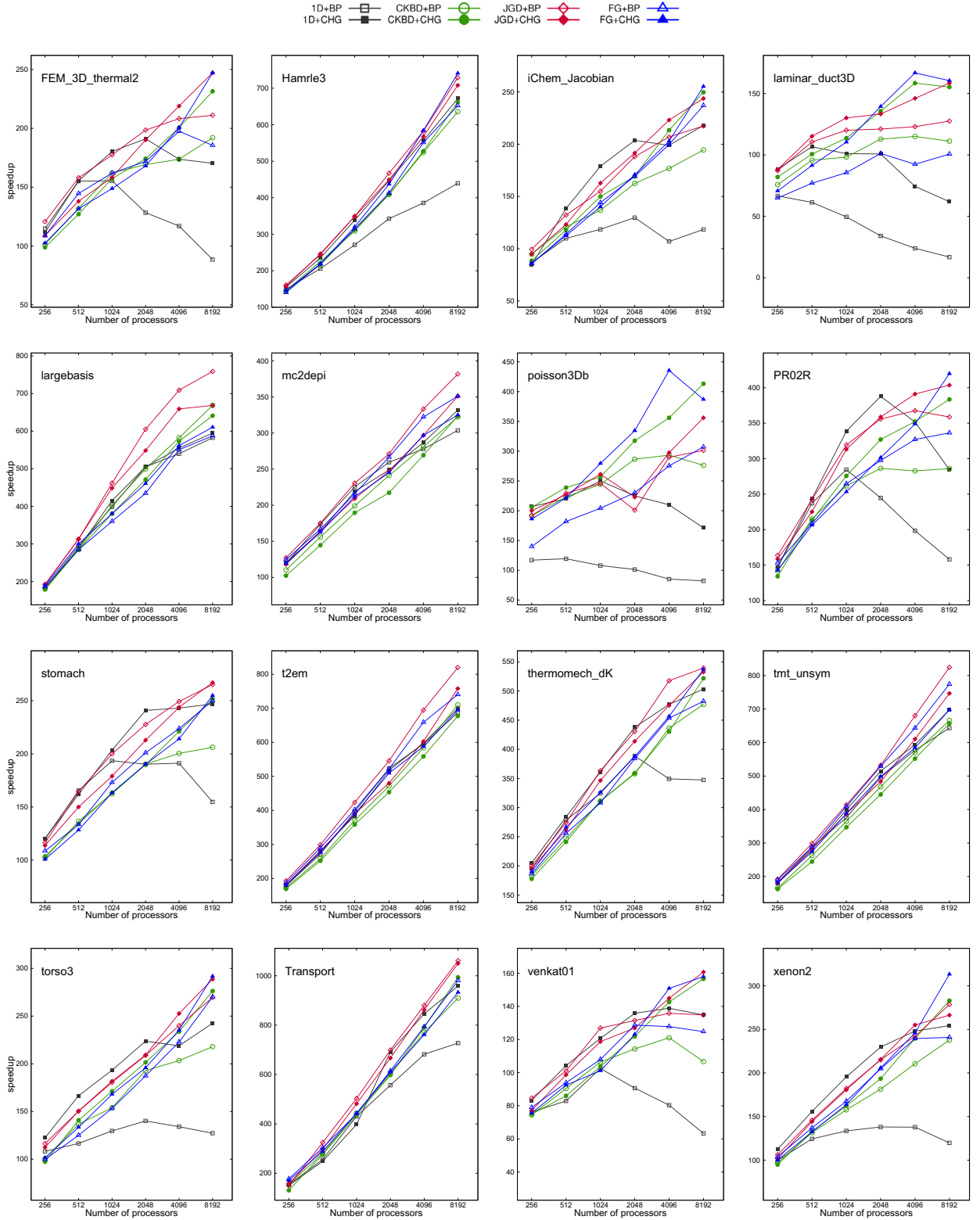
Fig. G12. Speedup curves for the remaining 16 matrices.
