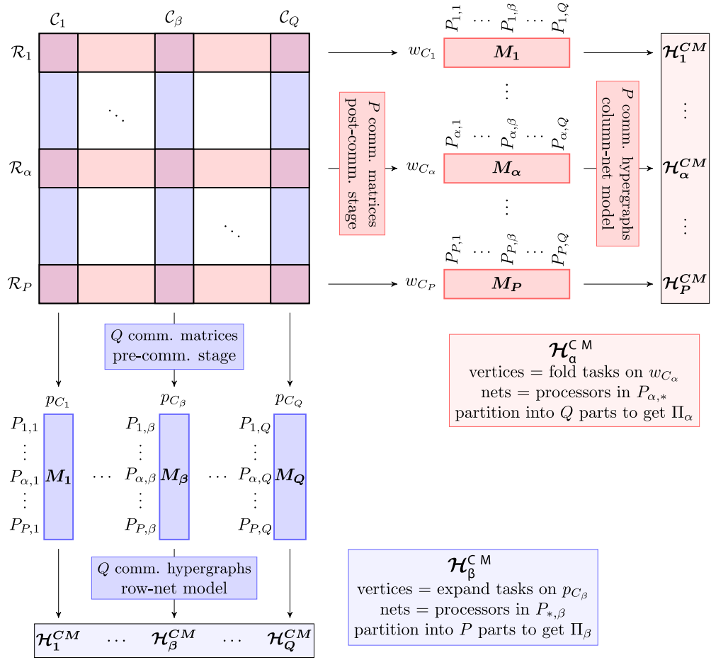
Fig. 4. Minimizing latency cost in checkerboard partitioning model.
