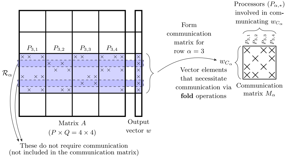
Fig. 3. Formation of the communication matrix for the third row of the processor mesh ( \alpha = 3 ) to summarize fold operations in the post-communication stage.
