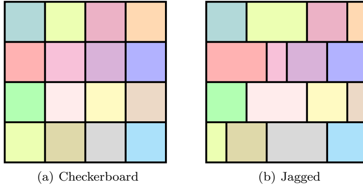
Fig. 1. A sample of 2D checkerboard and jagged partitionings on a 16 = 4 \times 4 virtual processor mesh.
