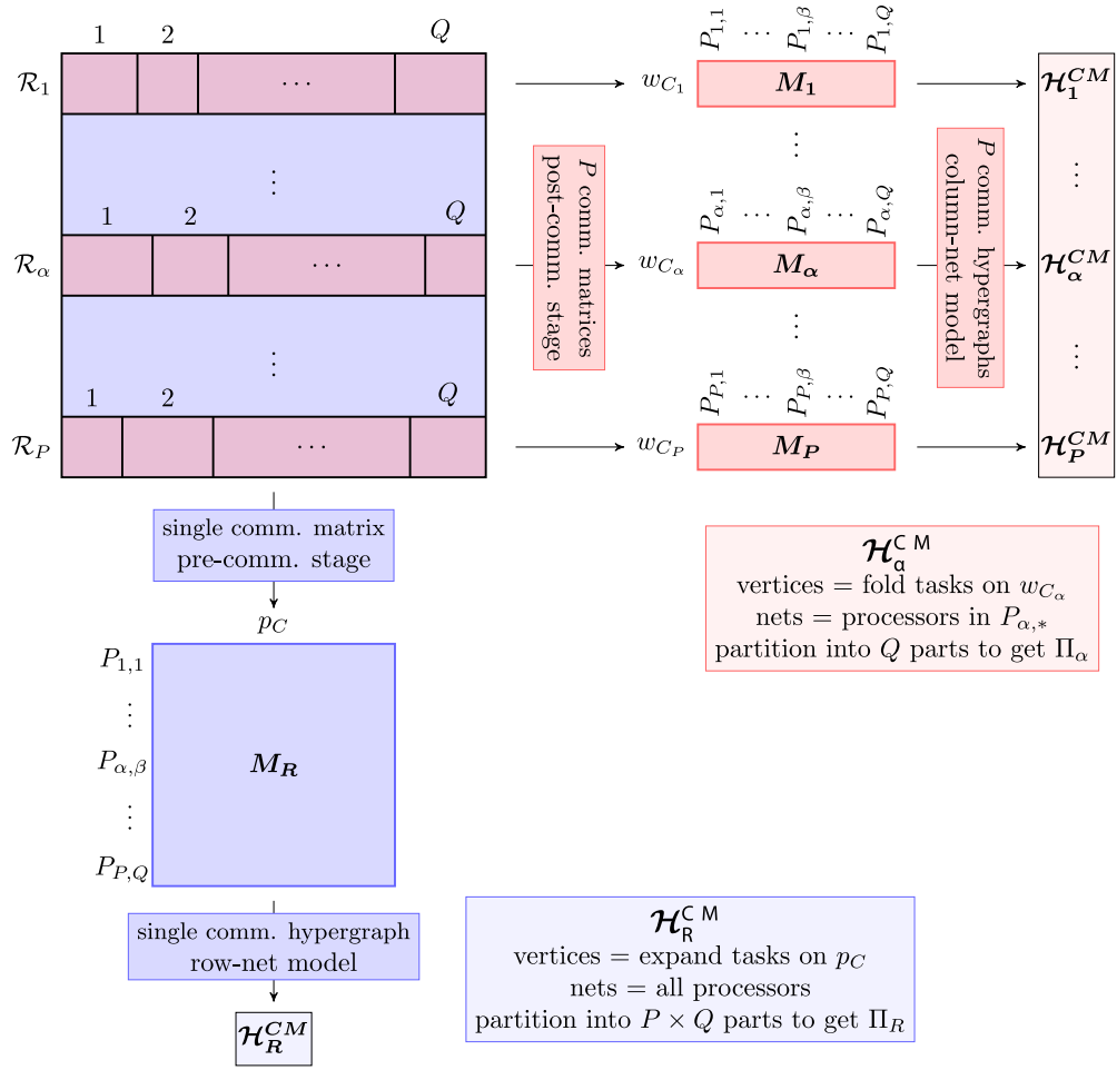
Fig. 5. Minimizing latency cost in jagged partitioning model.
