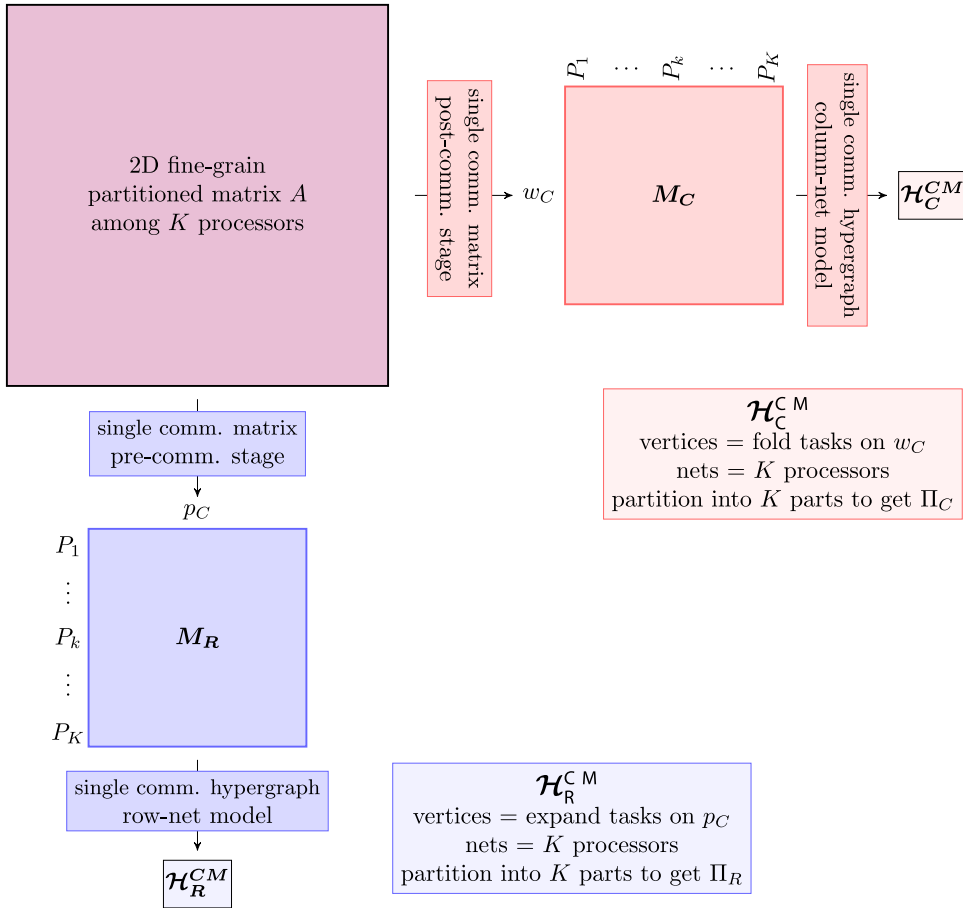
Fig. 6. Minimizing latency cost in fine-grain partitioning model.
