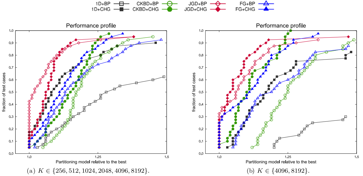
Fig. 8. Runtime performance profiles of eight partitioning models.
