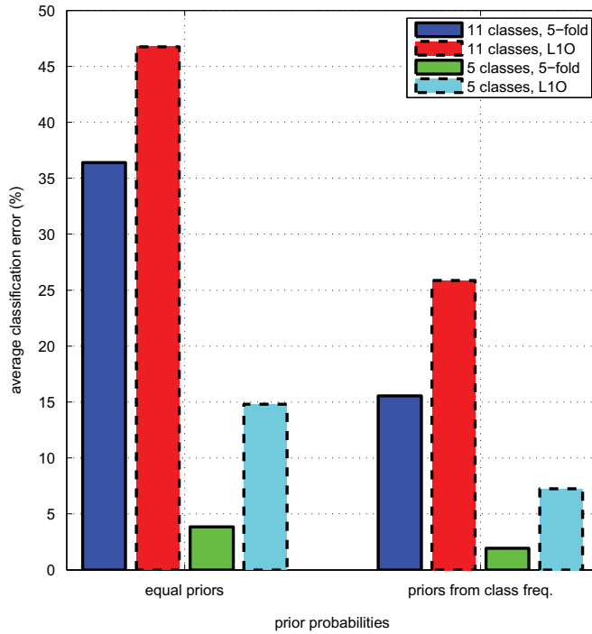
Figure 11. Effect of prior probabilities on the average classification error of the k -NN classifier (classifier 6).
