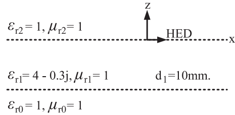
Fig. 7. Lossy dielectric material in air at f = 4 GHz.
