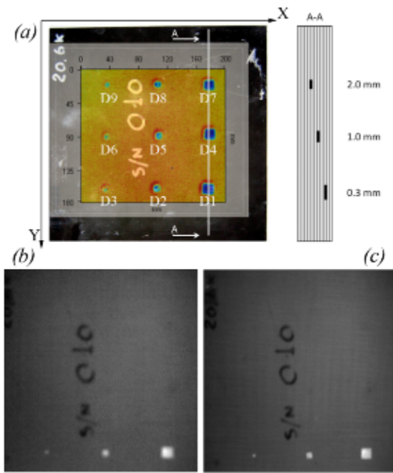
Fig. 1. Ultrasonic C-scan (a); thermal image acquired by 320x240 FPA at t=0.1 s after heat pulse (b); thermal image acquired by 1024x768 FPA at t=0.1 s after heat pulse (c).
