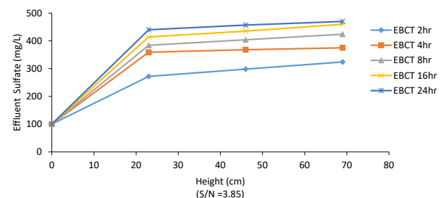
Figure 8. Effects of height and EBCT on effluent sulfate concentration.
