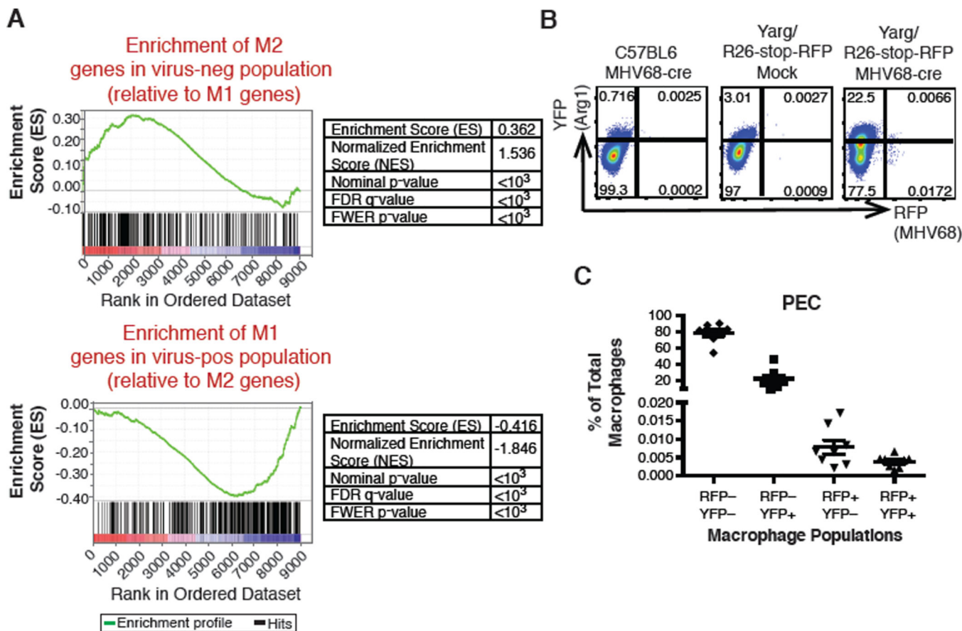
Fig. 2. IL-4 and IFN \gamma signatures identified in different macrophage populations during MHV68 infection
