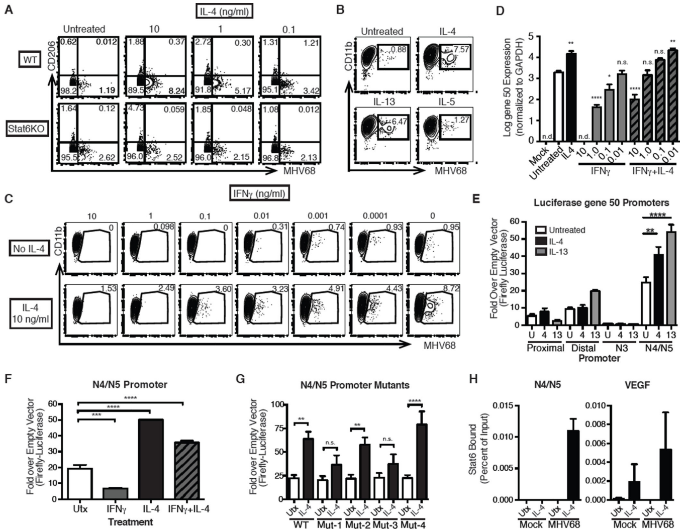
Fig. 3. IL-4 promotes viral replication and antagonizes IFN \gamma suppression of viral replication through direct binding to a viral promoter
