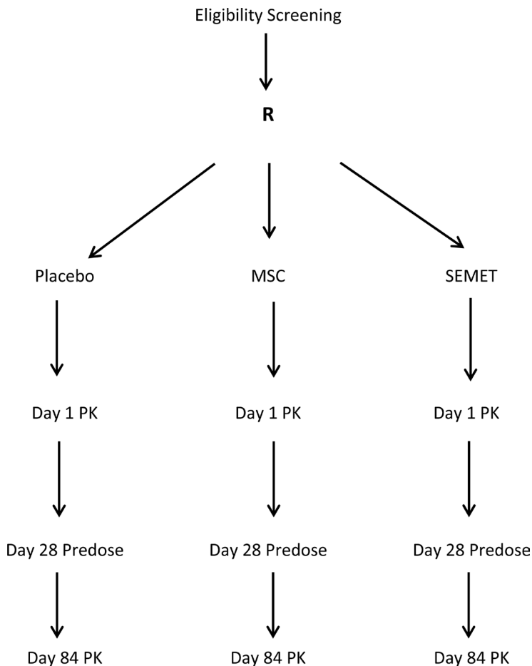
Figure 1: Phase 1 Multiple Dose Study of 12-week treatment by Se=Methyl-L-Selenocysteine (MSC) and L-Selenomethionine (SEMET) in adult males.
