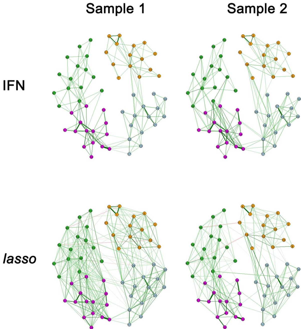
Figure 1. A visualization comparison of the WSS-SF networks structure for the samples of the IFN-based and lasso-based methods. Nodes are identified by color and scale: physical anhedonia (orange; 1-15), social anhedonia (blue; 16-30), perceptual aberration (purple; 31-45), and magical ideation (green; 46-60). Edge thickness depicts the strength of edge weights.
