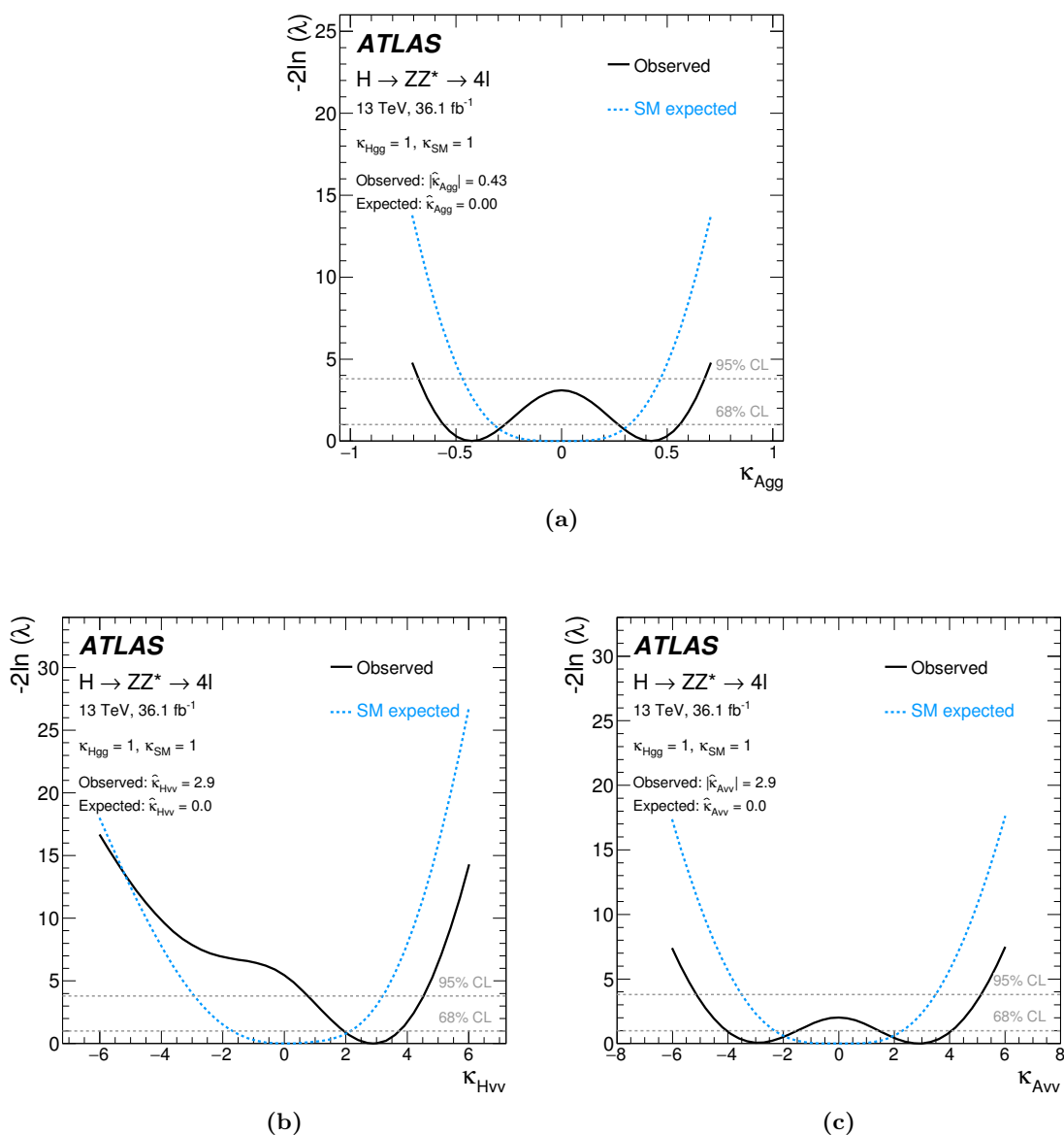
Figure 9. Observed (solid black line) and SM expected (dashed blue line) negative log-likelihood scans for (a) \kappa_{A_{gg}} , (b) \kappa_{H_{VV}} and (c) \kappa_{A_{VV}} coupling parameters using 36.1 fb -1 of data at \sqrt{s} = 13 TeV. The horizontal lines indicate the value of the profile likelihood ratio corresponding to the 68% and 95% CL intervals for the parameter of interest, assuming the asymptotic \chi^2 distribution of the test statistic.
