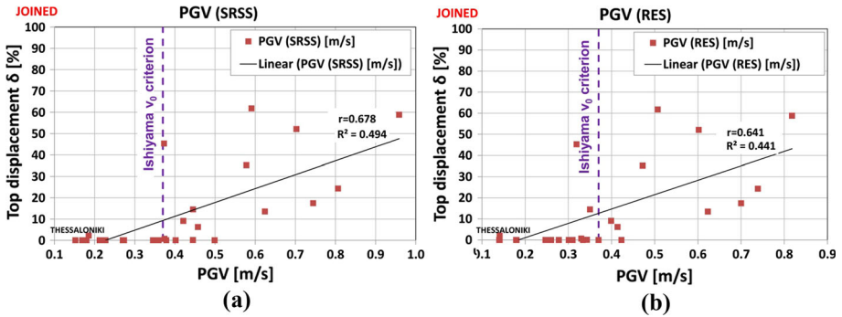
Fig. 13 Dispersion graphs of the independent variables PGV_{(SRSS)} and PGV_{(RES)} and the dependent variable \delta for the joined configuration
