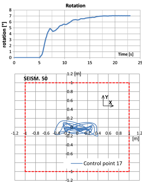
Fig. 7 Rotation time-history ( top ); displacement of control point 17 of the capital ( bottom ) and deformed shape ( right ) of joined configuration for earthquake #50
