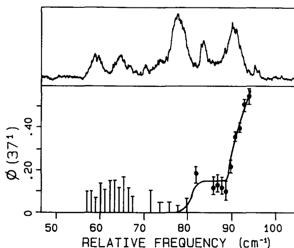
FIG. 7. A plot of the quantum yield of 37^1 production as a function of the excitation frequency over the broadened 36_0^1 37_0^1 -He and 37_0^2 -He contours. The error bars below 80 \text{cm}^{-1} in the figure denote upper bounds on the fractional 37^1 population since in these spectra only the 0^0 level is observed to within our signal to noise.
