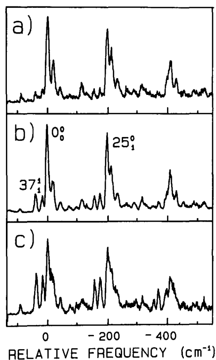
FIG. 6. Dispersed fluorescence spectra taken at three positions in the major broadened 37_0^2 transition. Excitation frequencies are (a) 88, (b) 90, and (c) 93 \text{cm}^{-1} above the origin. Note the dramatic change in the fraction of the emission due to the 37^1 level as one proceeds from (a)–(c).
