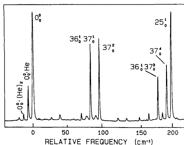
FIG. 1. Partially saturated laser-induced fluorescence excitation spectrum of trans -stilbene in the region near the S_1-S_0 origin under expansion conditions ( P_0 = 20 atm helium) in which stilbene-(He) _n complexes are present.
