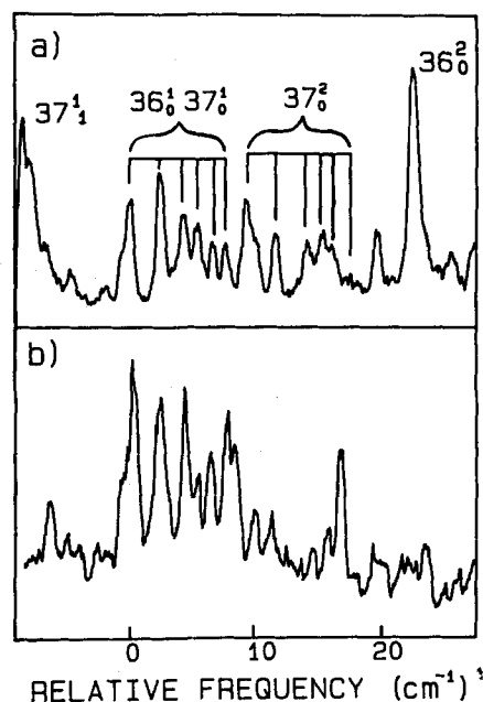
FIG. 11. Close-up fluorescence excitation spectrum (a) in the region of the 36_0^1 37_0^1 - \text{H}_2 and 37_0^2 - \text{H}_2 transitions, and (b) in the region of the 25_1^1 36_0^1 37_0^1 - \text{H}_2 and 25_1^1 37_0^2 - \text{H}_2 transitions. The tie lines indicate the substructure we have assigned to the 36_0^1 37_0^1 and 37_0^2 transitions.
