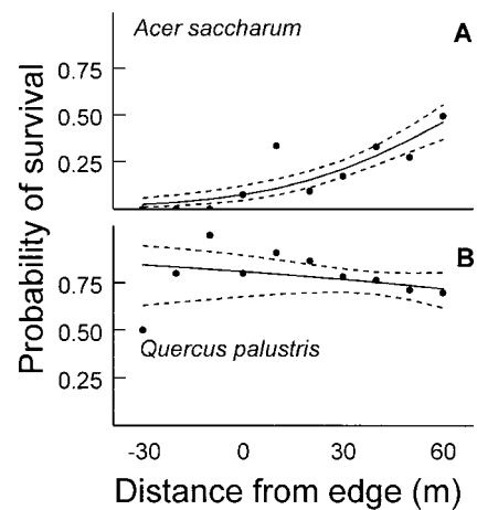
Fig. 3. Survivorship responses of Acer saccharum (A) and Quercus palustris (B) to the forest edge gradient. Negative distances from the edge (distance 0) indicate spatial positions inside the forest. Solid lines represent predicted probabilities of survival from a logistic regression, with dashed lines representing a 95% confidence interval around that prediction. Points represent proportion of emerged seedlings surviving to harvest at that distance.
