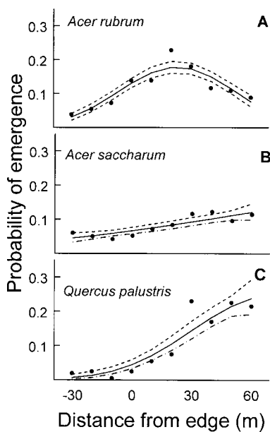
Fig. 2. Emergence responses of Acer rubrum (A), Acer saccharum (B), and Quercus palustris (C) to the forest edge gradient. Negative distances from the edge (distance 0) indicate spatial positions inside the forest. Solid lines represent predicted probabilities of emergence from a logistic regression, with dashed lines representing a 95% confidence interval around that prediction. Points represent proportion of planted seed emerging at that distance.
