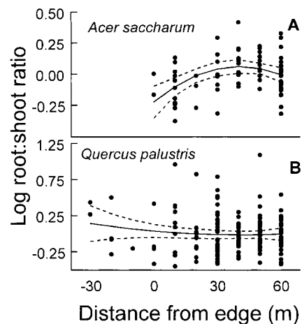
Fig. 6. Allocation responses of Acer saccharum and Quercus palustris to the forest edge gradient. Negative distances from the edge (distance 0) indicate spatial positions inside the forest. Solid lines represent predicted root : shoot ratio from a regression model, with dashed lines representing a 95% confidence interval around that prediction.
