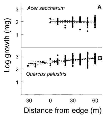
Fig. 5. Growth responses of Acer saccharum and Quercus palustris to the forest edge gradient. Negative distances from the edge (distance 0) indicate spatial positions inside the forest. Solid lines represent predicted growth from a regression model, with dashed lines representing a 95% confidence interval around that prediction.
