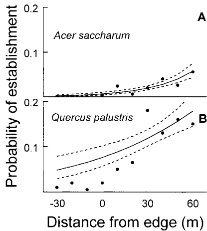
Fig. 4. Effect of the forest edge gradient on the establishment probabilities of Acer saccharum (A) and Quercus palustris (B). Negative distances from the edge (distance 0) indicate spatial positions inside the forest. Solid lines represent predicted probabilities of emergence from a logistic regression, with dashed lines representing a 95% confidence interval around that prediction. Points represent proportion of planted seed that became surviving seedlings at that distance.
