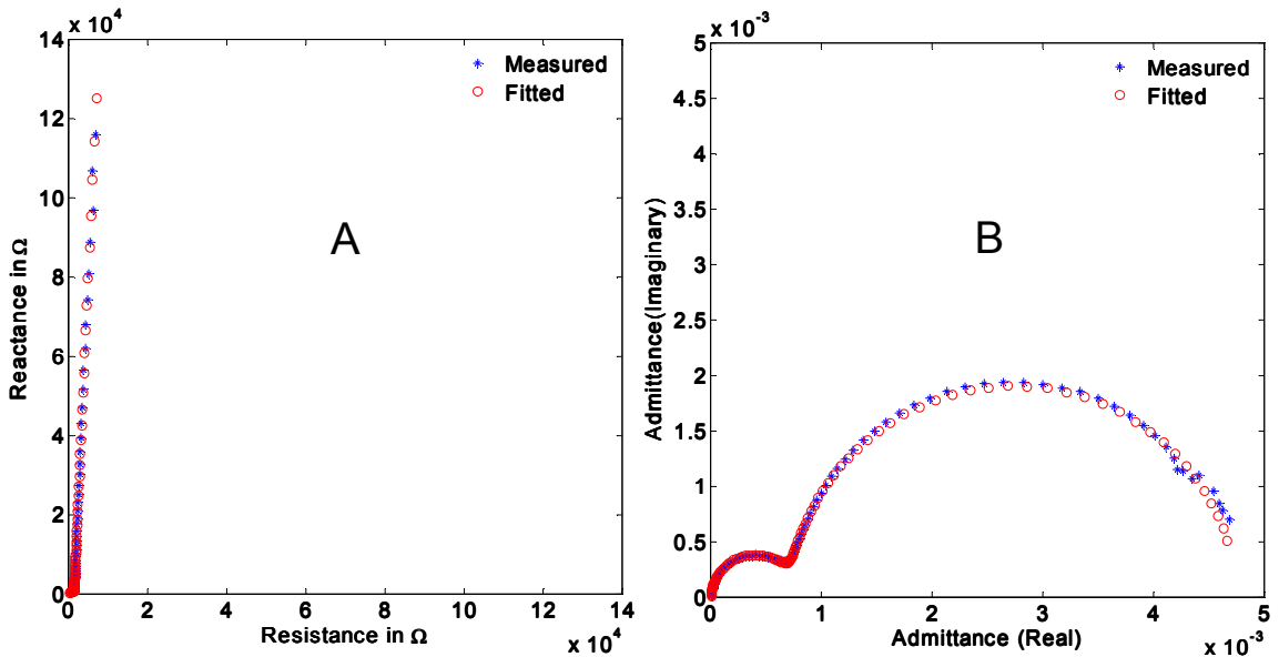
Figure 15: A) Complex plane impedance and B) Complex plane admittance plot of partially coated metal electrodes.
