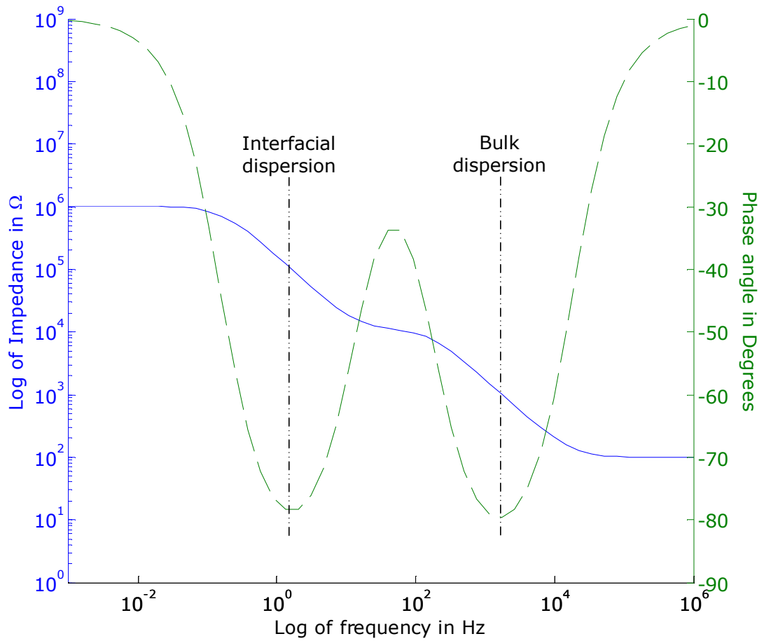
Figure 19: Bode diagram of a circuit approximating interfacial and bulk effects. R_b=1e4 , C_b=1e-7 , R_{ct}=1e6 , C_{dl}=1e-6 , R_s=1e2 .
