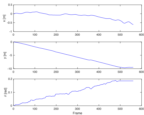
Fig. 12. The smoothed attitude-trajectory of 560 frames in the first track along the ship's hull.
