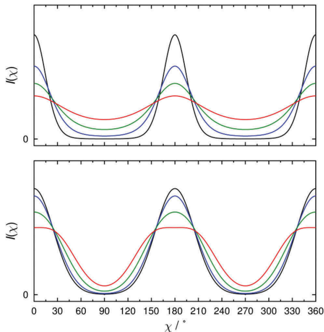
Figure 12. (Colour online) Calculated intensity profiles, I(\chi) , obtained from the maximum entropy distributions (top) and the sugar-loaf and diffuse-cone distributions (bottom) by numerical integration of Equation (5). The curves are coloured to match the distributions given in Figure 11.
