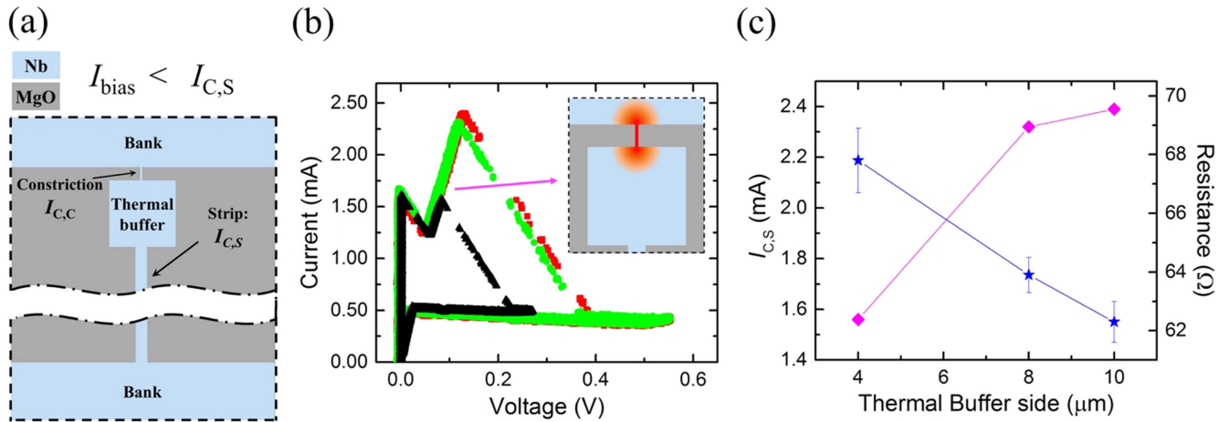
Figure 1. (a) Sketch of the proposed design for the single strip connected to the constrictions via a superconducting thermal buffer. (b) Graph showing the I-V characteristic, measured at a temperature of 4.2 K, for the strips having thermal buffer area of 4 \times 4 \mu m^2 (black triangles), 8 \times 8 \mu m^2 (green circles) and 10 \times 10 \mu m^2 (red squares). The inset illustrates the propagation of the normal resistive region in the thermal buffer when a bias current is in the range I_{C,C} < I_B < I_{C,S} . (c) Graph showing the values of the measured I_{C,S} (magenta diamonds) and of the resistances when the strips are biased in the range I_{C,C} < I_B < I_{C,S} (blue stars) as the thermal buffer side width varies.
