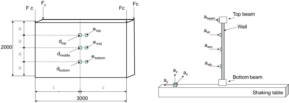
Figure 3 Instrumentation layout diagram. Left: panel front view showing displacement transducers, strain gauges and load cell positions. Right: panel side view showing accelerometers on the wall and on the shaking table platform.
