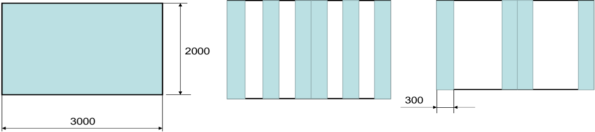
Figure 1 Layouts of FRP fabric on the masonry panel. Left: continuous jacket (100% RR), middle: vertical strips (60% RR), right: vertical strips (40% RR). Reinforcement applied on both sides of the panel. (Note: RR stands for Reinforcement Ratio).
