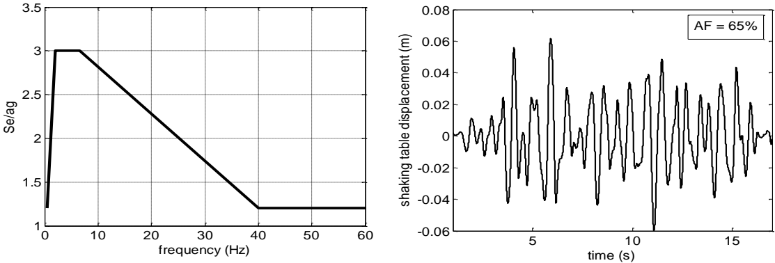
Figure 4 Design response spectrum acc. to Eurocode 8 (left) and matched shaking table displacement time history for AF=65% (right).
