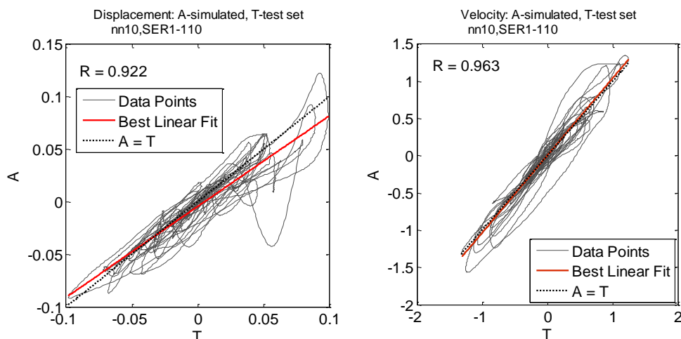
Figure 9 Regression analysis for the NN output (A) and the test set (T) for displacement, for panel SER1 (RR=100%) in test AF110% (R= regression coefficient).
