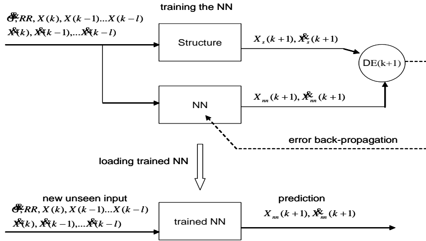
Figure 7 Neural network model for dynamic system identification: mode of operation
