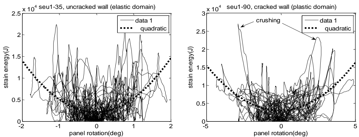
Figure 5 URM panel's average potential well at AF=35% (left) and AF=90% (right).
