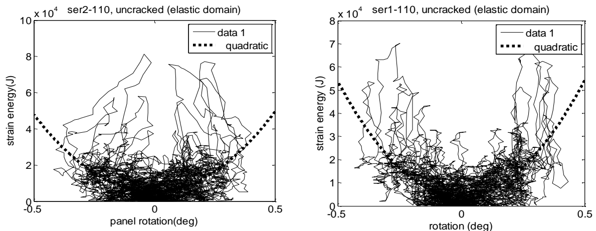
Figure 6 Average potential well for reinforced panels ((RR=60%, AF=110% left) and (RR=100%, AF=110% right)).
