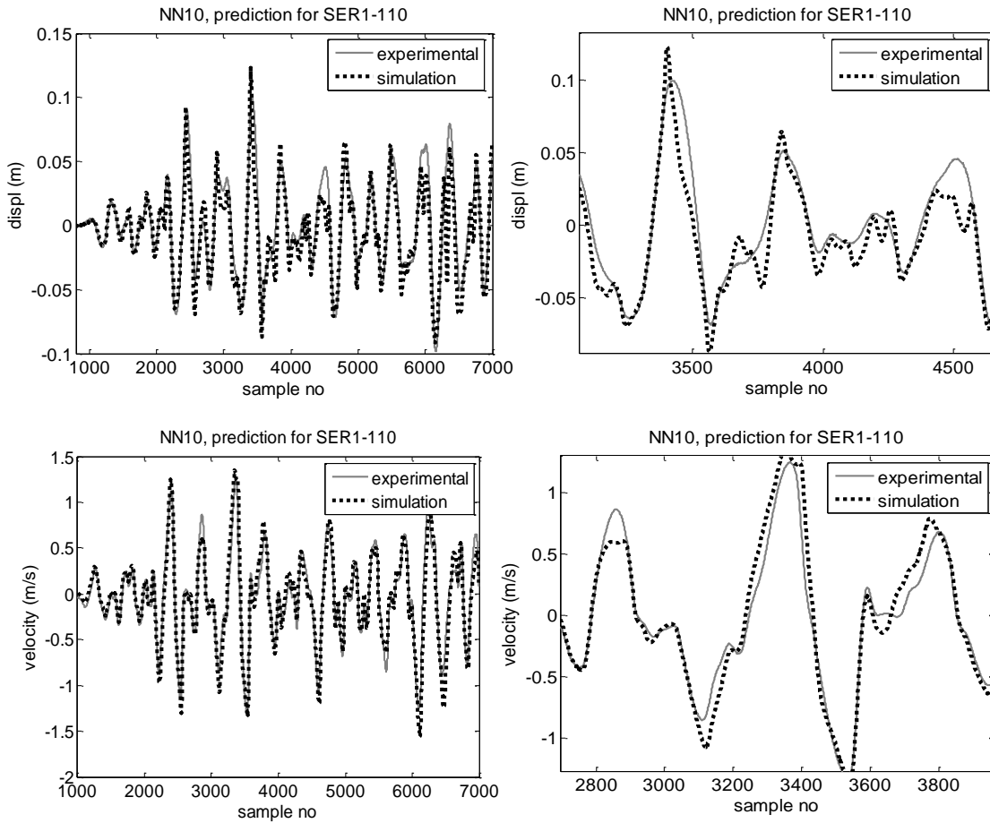
Figure 8 NN prediction and experimental measurements of out-of-plane displacement and velocity for panel SER1 (RR=100%) in test AF1 10%, after 20000 epochs of training.
