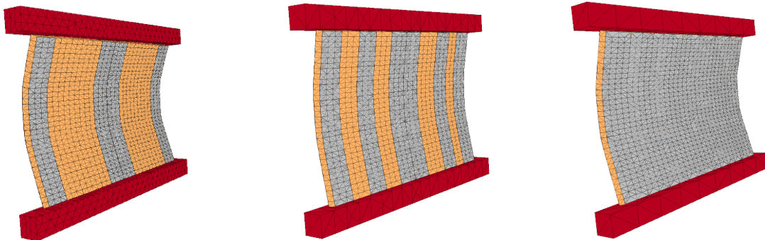
Figure 12 Failure patterns from the numerical model. Left: vertical strips (40% RR), middle: vertical strips (60% RR), right: continuous jacket (100% RR). Reinforcement is applied on both sides of the panel. (Note: RR stands for Reinforcement Ratio).
