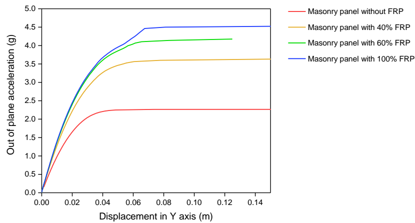
Figure 13 Pushover curves for the masonry panel with different reinforcement percentages
