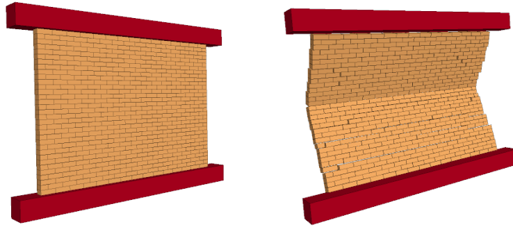
(a) Numerical model of masonry panel in 3DEC (b) Out-of-plane failure for masonry panel Figure 10 Numerical simulation in 3DEC for the masonry panel under out-of-plane loading.
