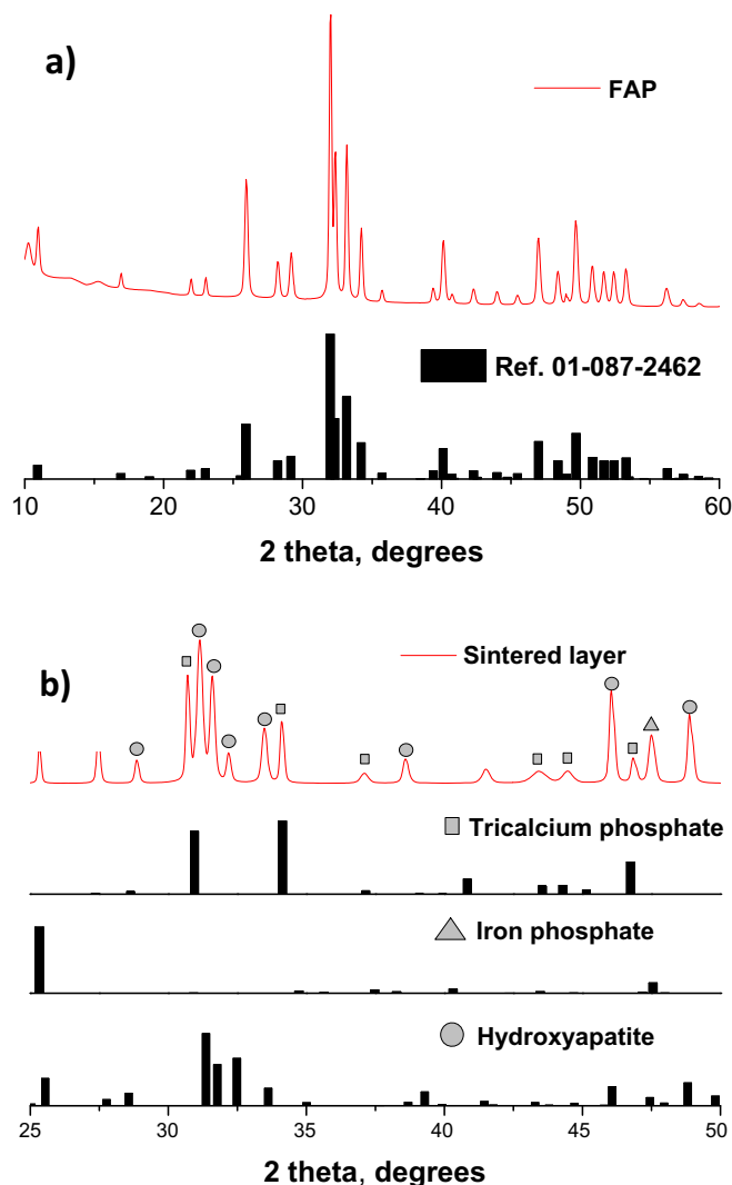
Fig. 1. X-Ray diffraction patterns of a) the as-synthesized fluorapatite powder (after heat treatment); b) laser-sintered Fe-containing fluorapatite coating on enamel surface. Reference patterns of phases identified in the experimental patterns are shown below.
