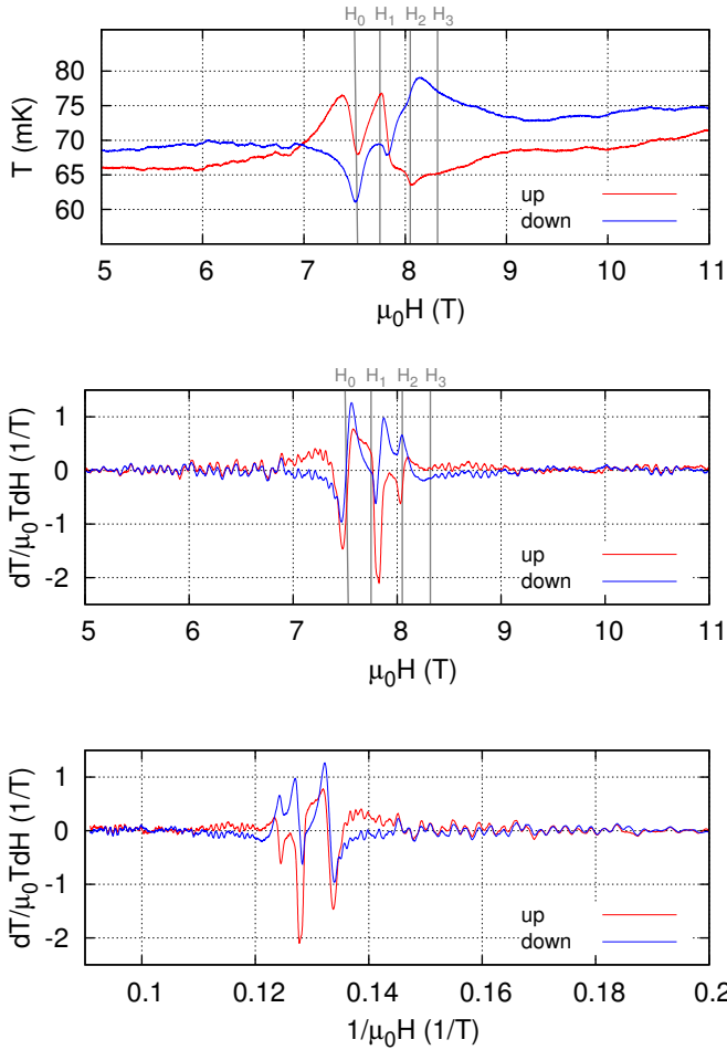
FIG. 5. In the upper panel we show exemplary raw data of magnetocaloric sweeps between 5 and 11 T using the quasi-adiabatic method. Strong signatures can be seen at H_0 , H_1 and H_2 , and a weak kink at H_3 emphasized in Fig. 4c. Below 7 T and above 9 T, i.e. outside the critical region, quantum oscillations are visible on this data. In the middle panel we show the field derivative of the same data, which are plotted over 1/H in the lower panel.
