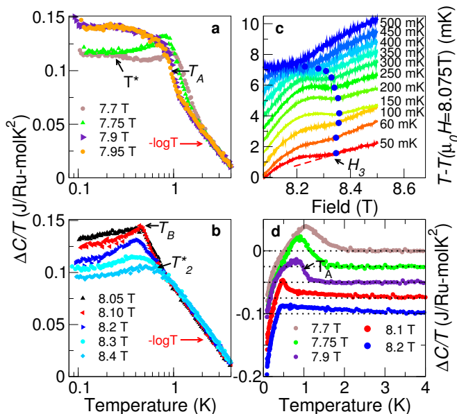
FIG. 4. (a) The electronic specific heat coefficient \Delta C/T as a function of the temperature at 7.7, 7.75, 7.9 and 7.95 T in the vicinity of the A phase, and (b) at 8.05, 8.1, 8.2, 8.3 and 8.4 T, in the vicinity of the B phase. (c) Magnetocaloric data for 8.075 \leq \mu_0 H \leq 8.5 T and 0.05 \leq T \leq 0.5 K. The blue circles mark the locations H_3 of a weak feature (kink) that we tentatively associate with the boundary of the B phase, but the data show no obvious signature of a phase transition. (d) \Delta C/T across the region of phase formation after subtraction of the logarithmically diverging background signal extrapolated to low temperatures, following the procedure described in the main text. The data including this background are shown for 7.7 to 8.2 T in Figs. 4a,b. The data in the plot are shifted for clarity.
