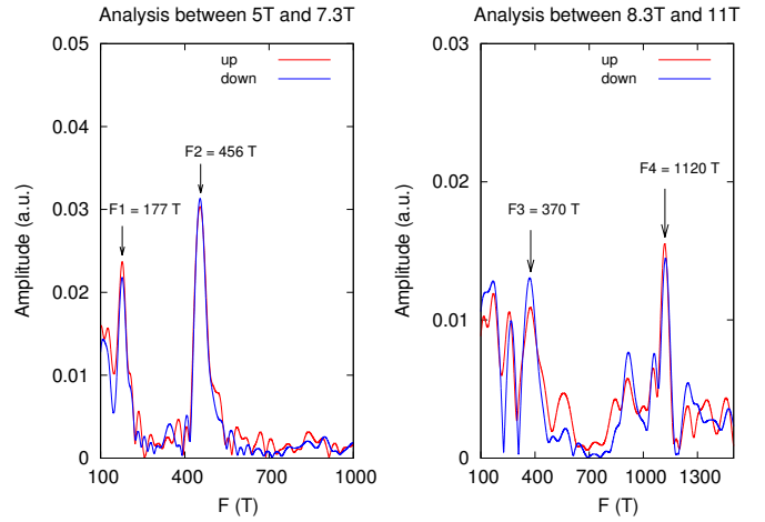
FIG. 6. Fourier analysis of the data shown in Fig. 5. The main frequencies are the 456 T in the low-field region and 1120 T in the high-field region.
