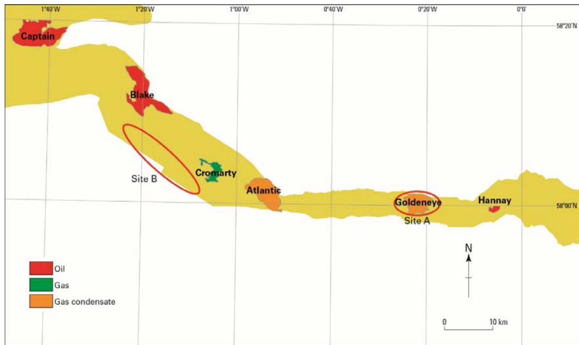
Fig. 2. The eastern part of the area of the Captain Sandstone shown in Fig. 1 investigated as a case study for the operation of a multi-user CO 2 storage formation showing the position of Site A and Site B for dynamic modelling of CO 2 injection, hydrocarbon fields within the Captain Sandstone, and lines of latitude and longitude.
