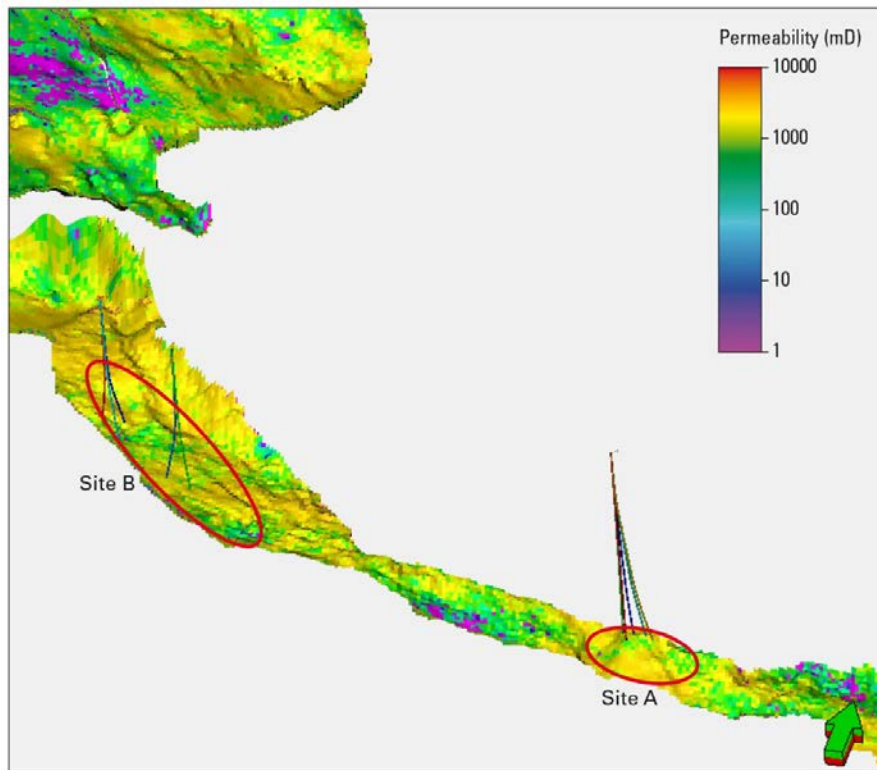
Fig. 5. Permeability model of the eastern extension of the CO 2 MultiStore Captain Model used for dynamic simulation of CO 2 injection showing the position of injection Site A and Site B, and the position and trajectory of the wells modelled for CO 2 injection at each site. Permeability values in milliDarcy, mD.
