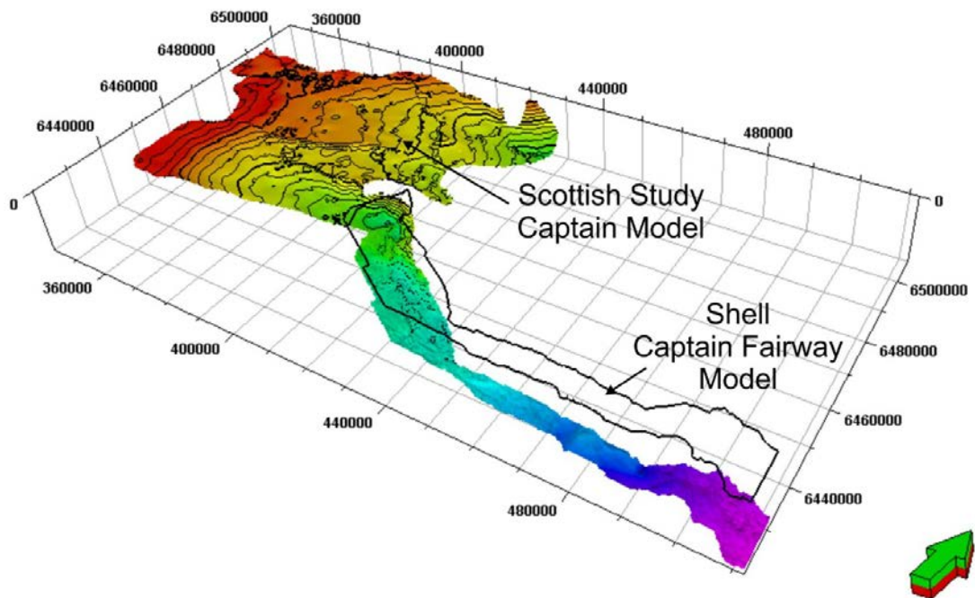
Fig. 3. Three-dimensional image of the upper surface of the CO 2 MultiStore Captain Model from two existing merged geological models [5,6], outline of [6] shown with black polygon.
