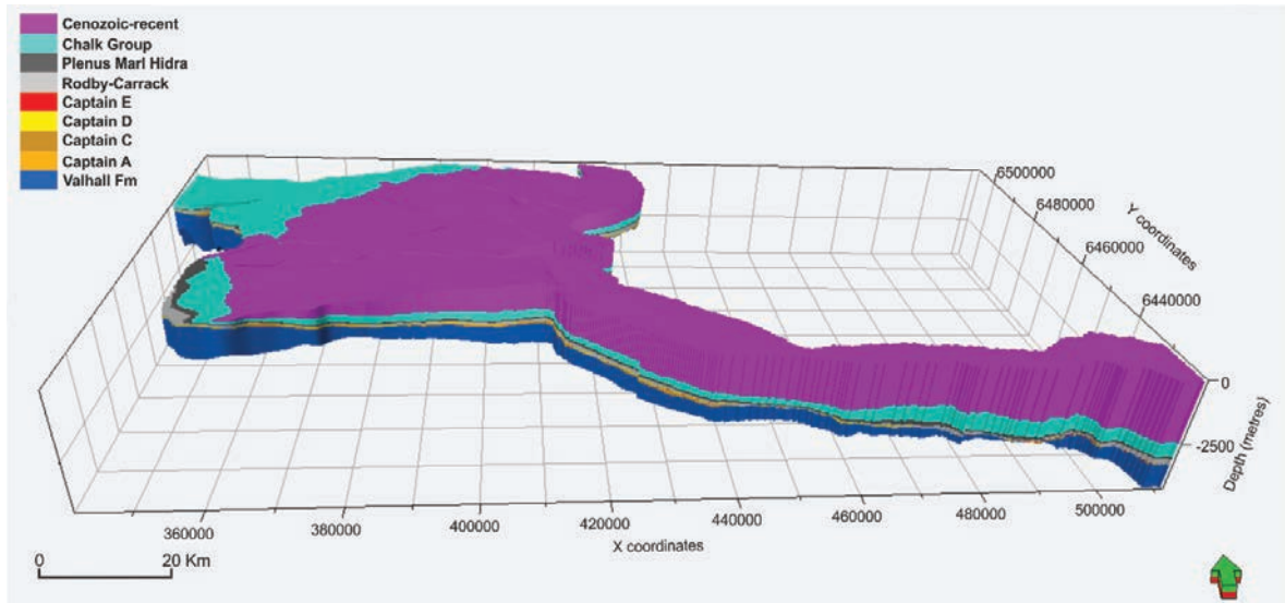
Fig. 4. Geological CO 2 MultiStore Captain Model (approximately 163 km from west to east, 84 km from north to south and with an area of approximately 8000 km 2 ) illustrating the nine intervals modelled from the sea bed down to the rocks underlying the Captain Sandstone
