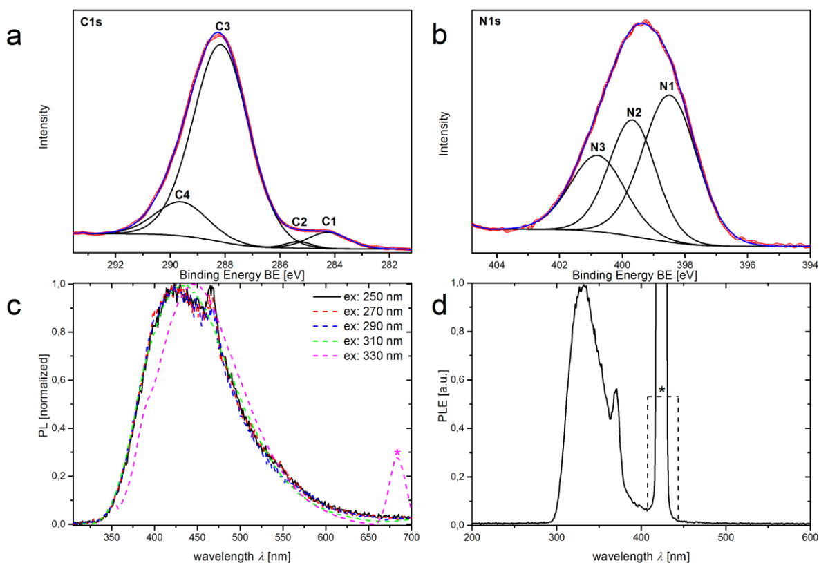
Figure 4 C1s (a) and N1s (b) XP spectra of PTI. Red circles denote the measured data and the fits are represented by blue curves. With an increasing excitation wavelength the photoluminescence spectra of PTI in NaOH solution (pH 12) shows a redshift in the photoluminescence (c). The PLE spectrum shows two maxima. The first and more intense is found at 330 nm and is contributed by PTI, the second at 370 nm is assigned to Raman scattering of water (d). The asterisks in (c) and (d) mark measurement artefacts at double excitation wavelength and the excitation wavelength, respectively.
