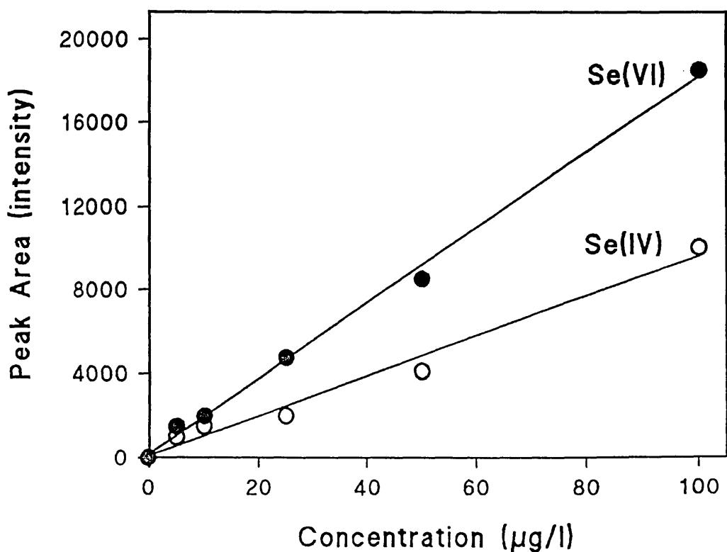
Fig. 20. Calibration graphs for selenium(VI) and selenium(IV), based on processing 10 ml of sample.
