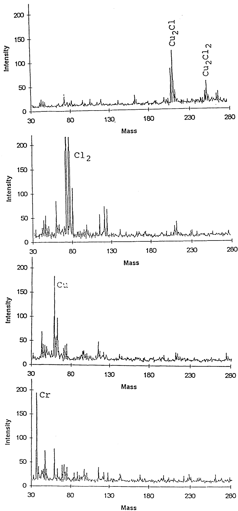
Fig. 25 Mass scans of the range 30-280 amu taken during the vaporisation of the mixture of copper nitrate and chromium chloride (10 \mu\text{l} ). Each spectra has a 0.15 seconds difference.
