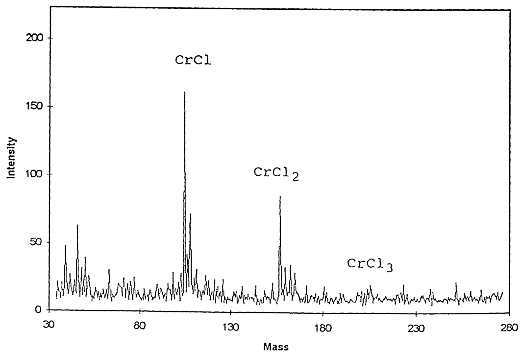
Fig. 24 Scan of the mass range 30-280 amu while vaporising (a) Copper (II) Nitrate (10ppm, 10 \mu\text{l} ) and (b) Chromium (III) Chloride (10ppm, 10 \mu\text{l} ).
