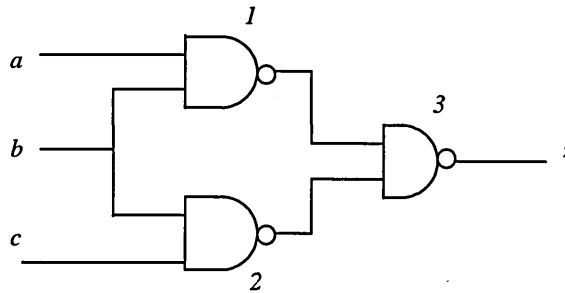
Figure 1.11: z = \overline{\overline{ab}.bc}
