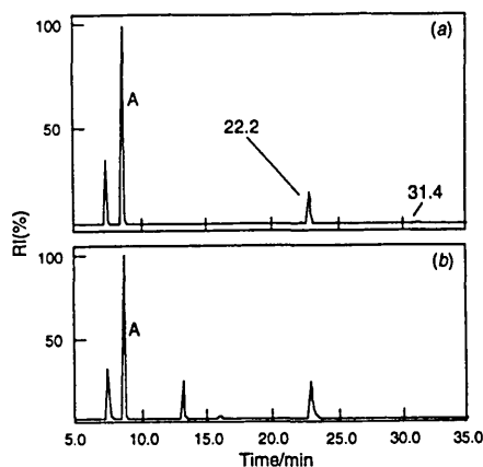
Fig. 2 Total ion current chromatograms for the (a), methanolic and (b), etheral extracts of products from the uncatalysed autoclave oxidation of 2-picoline. A, 2-picoline \times 29
