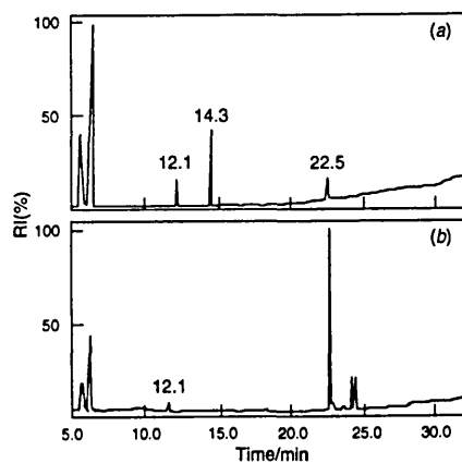
Fig. 3 Total ion current chromatograms for the (a), methanolic and (b), etheral extracts of products from the Fenton catalysed autoclave oxidation of 2-picoline
