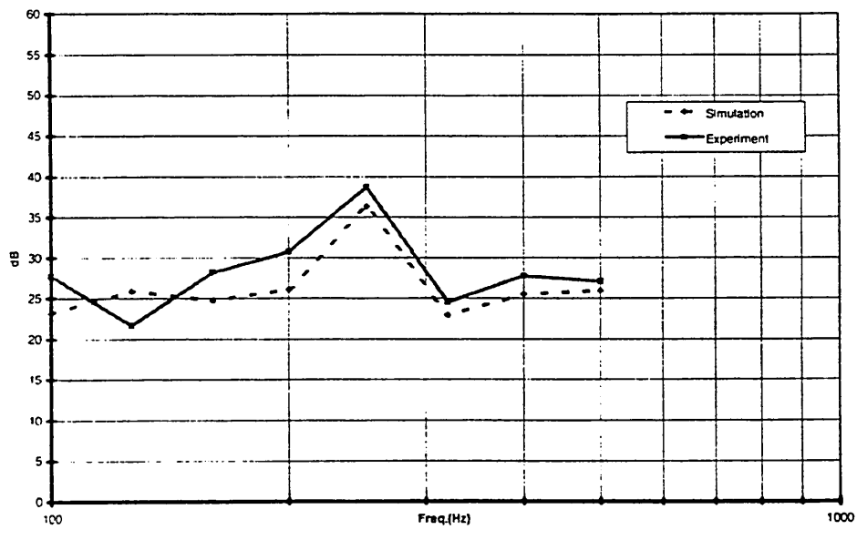
Figure 11. Sound pressure level difference calculated for a 10 mm perspex sheet.
