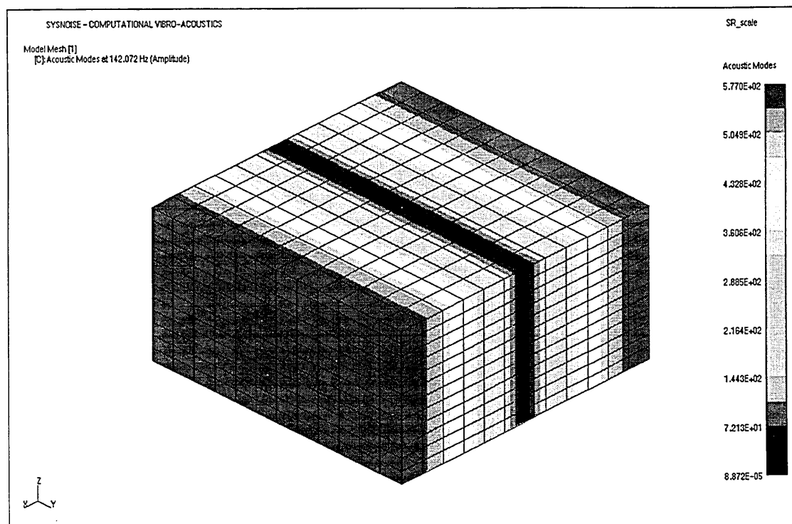
Figure 3.2. Axial mode (1,0,0)
