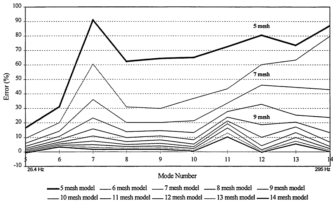
Figure 6.7. Structural model : Error versus Mode
