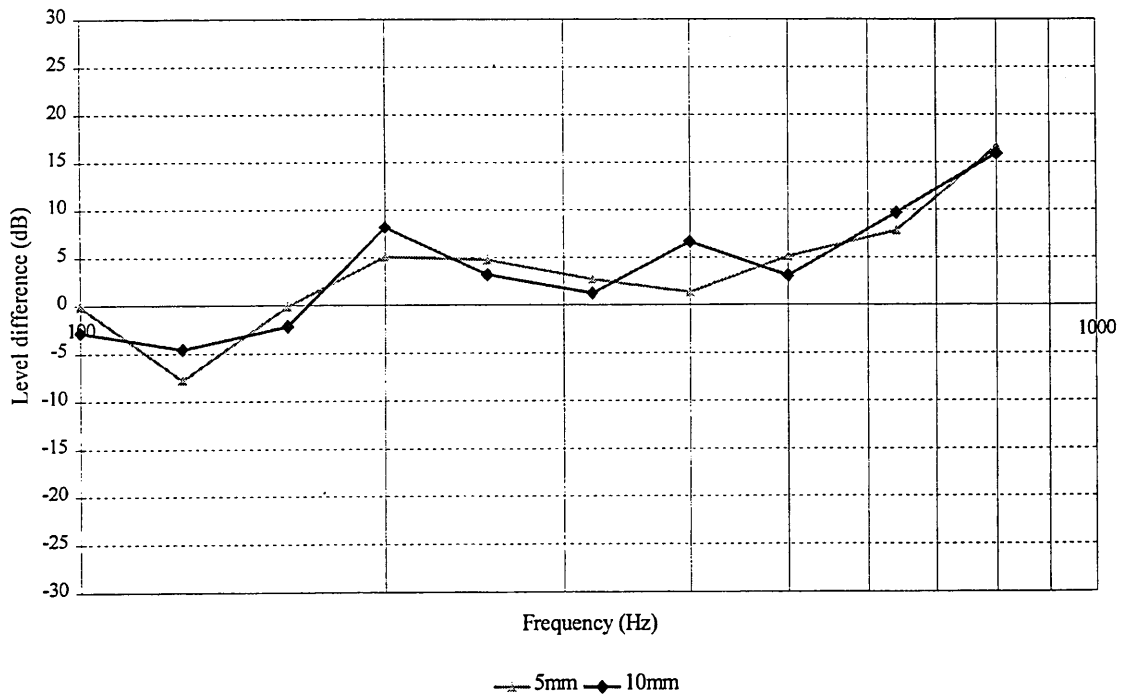
Figure 8.33. Positions 1 and 4: Measured sound pressure level difference compared with predicted level difference in a 1/3 octave band
