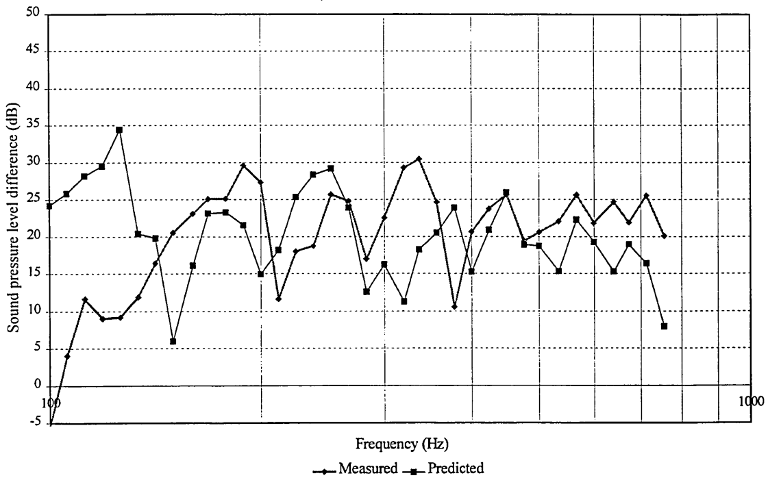
Figure 8.21. Sound level difference between averaged positions of a 5mm panel in a 1/12 octave band
