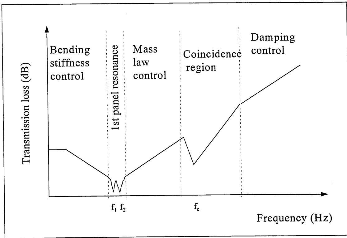
Figure 2.1. Transmission loss versus frequency
