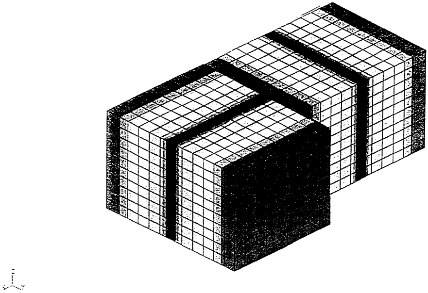
Figure 9.35. Excitation of the first acoustic axial mode in the asymmetric transmission rooms
