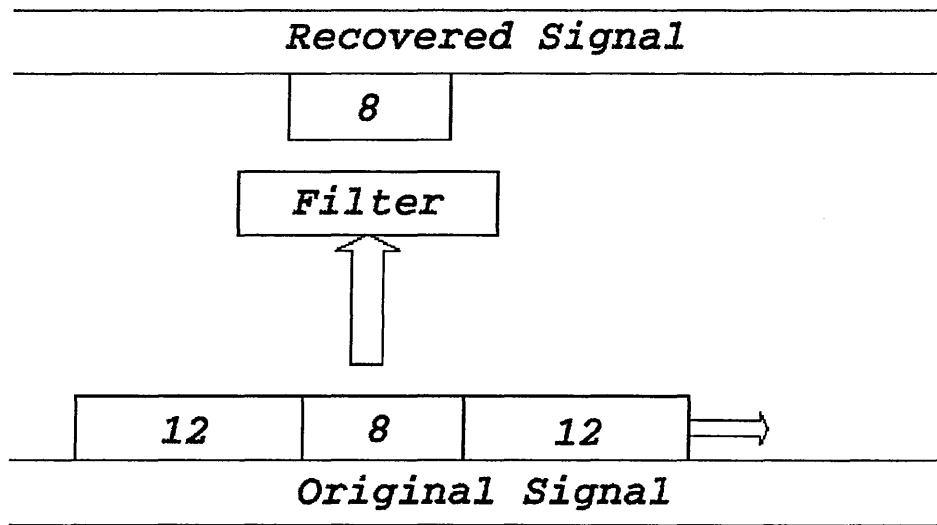
Figure 4.4: The sliding window technique
