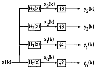
Fig. 2 Tree-structured analysis filter bank
