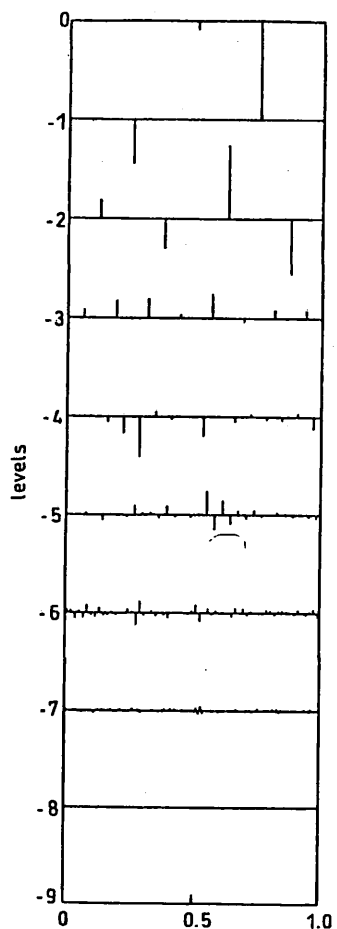
Fig. 16 Spike plot of MRA coefficients for Fig. 10
