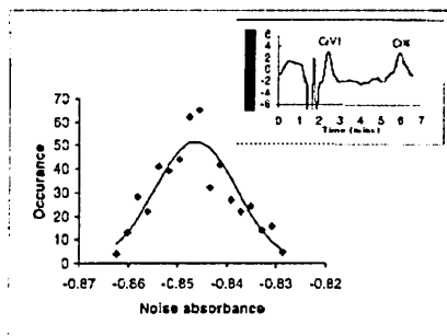
Figure 5. Chromatogram of solution containing 0.05 \mu\text{g L}^{-1} Cr(III) and Cr(VI) (inset), and least-squares Gaussian fit of the baseline fluctuation.
