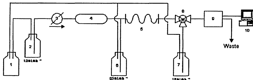
Figure 1. Schematic diagram of the ion chromatography system with chemiluminescence detection.
