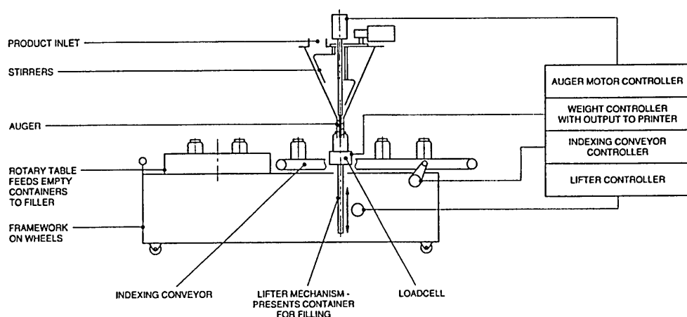
Figure 95: Fully automated filling machine type DM1 (taken from Kramer et al. [242] ).
