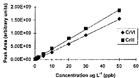
Figure 4. Calibration graphs for Cr(III) (■), y = 4.0 \times 10^7 x - 2.0 \times 10^7 , and Cr(VI) (◆), y = 3.0 \times 10^7 x - 2.0 \times 10^7 , in the concentration range 0.01–50 \mu\text{g L}^{-1} .
