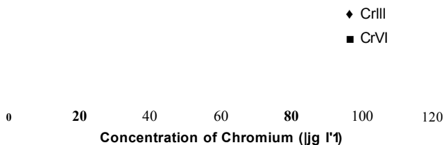
Figure 58: CrIII/VI calibration graph showing the effect of Cr(III) adsorption to glass autosampler vials using IC-CL.
