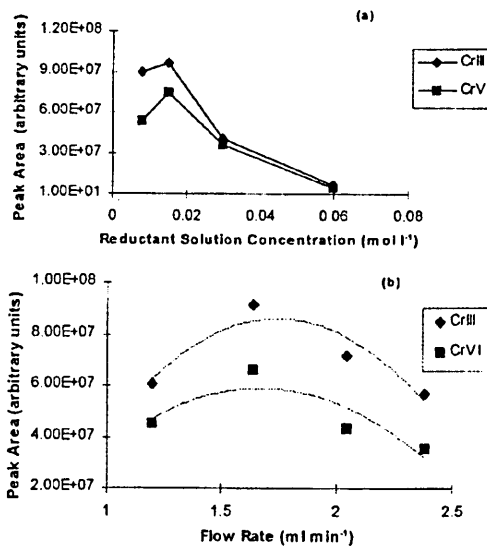
Figure 3. (a) Effect of varying reductant solution concentration on the Cr(III) (◆) and Cr(VI) (■) chemiluminescence signals. (b) Effect of luminal flow rate on the chemiluminescent signal intensities of Cr(III) (◆) and Cr(VI) (■).
