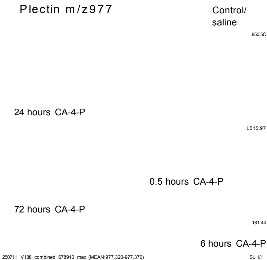
Figure 4. 44: MALDI-MSI multiple Fibrosarcoma 188 sample on tissue digest of Plectin at m/z 977.
