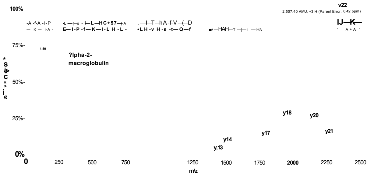
Figure 3. 35: MS/MS spectrum and normalised intensity graph of Alpha-2-macroglobulin in fibrosarcoma 188 LC-ESI-MS/MS results. Insert displays the normalised spectral counts for Alpha-2-macroglobulin throughout the time course post CA-4-P.
