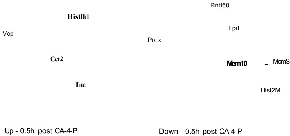
Figure 4. 41: iTRAQ proteomic response results using a 0.5h post CA-4-P Fibrosarcoma 188 treatment. The proteins in the 'Up' 0.5h time point do not have any associations here, in the 'Down' group a strong associative link is present between Mcm10 and Mcm5 with a weaker relationship clear between Prdxl and Tpil.
