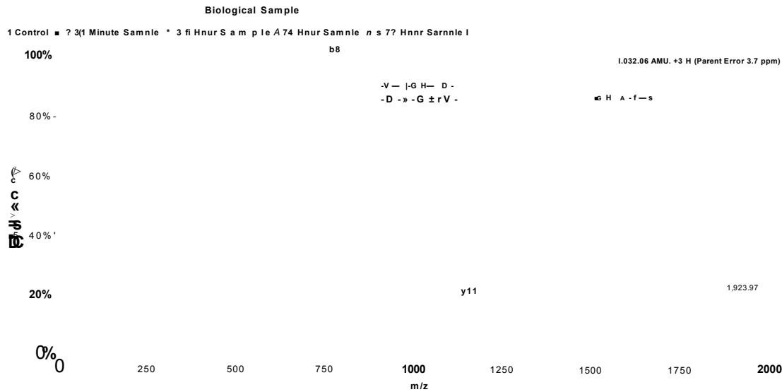
Figure 3. 43: Example MS/MS spectrum and normalised intensity graph of Alpha-enolase in fibrosarcoma 188 LC-ESI-MS/MS results. Insert displays the normalised spectral counts for Alpha-enolase throughout the time course post CA-4-P.
