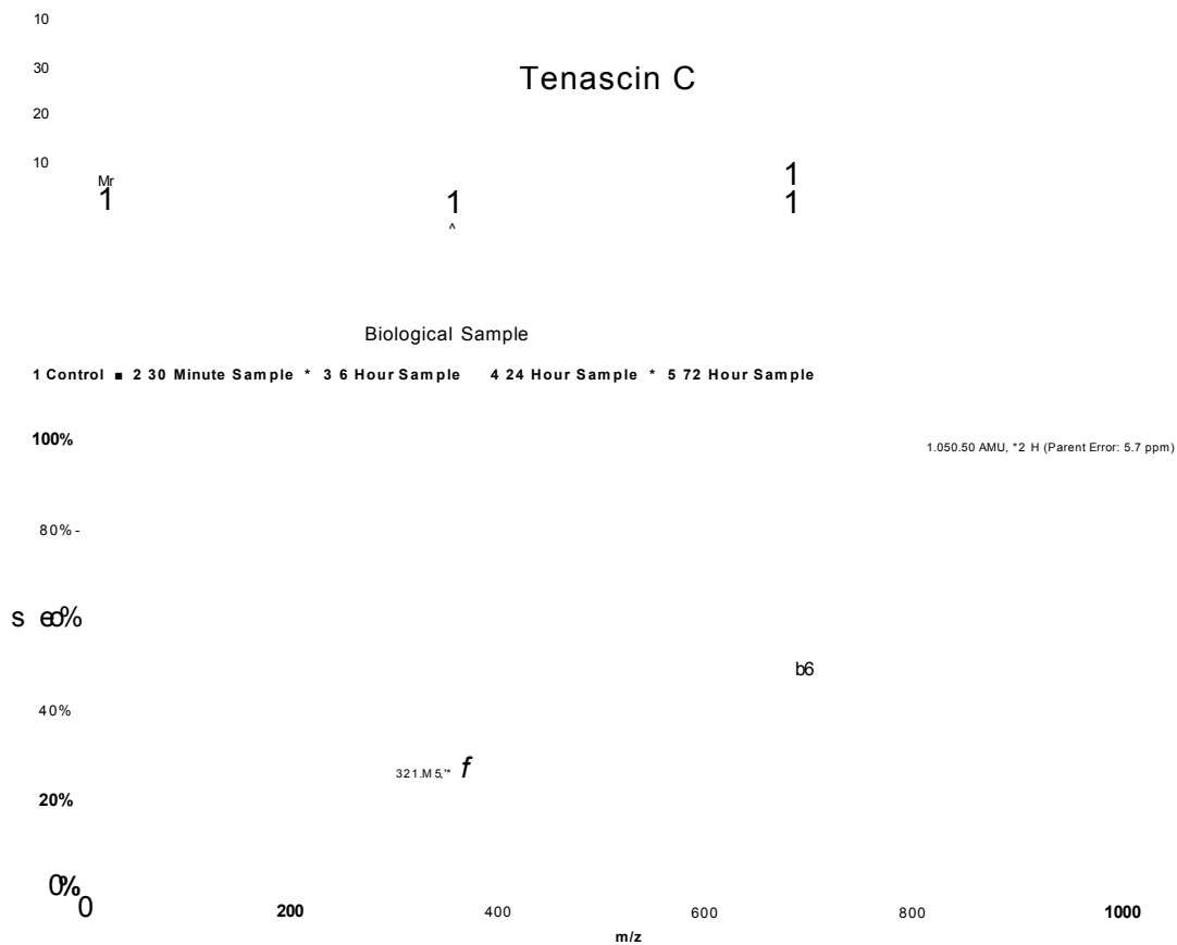
Figure 3. 42: Example MS/MS spectrum and normalised intensity graph of Tenascin C in fibrosarcoma 188 LC-ESI-MS/MS results. Insert displays the normalised spectral counts for Tenascin C throughout the time course post CA-4-P.
