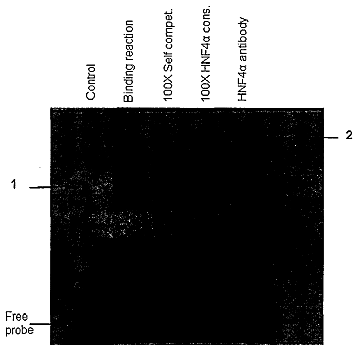
Fig 3.24. Supershift assay and competitive EMSA using the pZHNH4 \alpha -fluorescent binding site. Control was the pHNH4 \alpha probe (-48/-38) without HepG2 NE. Binding reaction was the pZHNH4 \alpha probe (-48/-38) with HepG2 nuclear extract (Hep NE). Self competitor was the pZHNH4 \alpha probe, the HepG2 NE and the unlabeled pZHNH4 \alpha . HNF4 \alpha consensus lane was the pZHNH4 \alpha probe, the HepG2 NE and unlabeled HNF4 \alpha binding consensus. HNF4 \alpha antibody lane contained the pZHNH4 \alpha probe, the HepG2 NE and the HNF4 \alpha antibody. Bands indicated by arrow 1 represent protein DNA complexes. Band 2 represents the potential antibody-protein-DNA complex. Competition is seen with 100-fold molar excess of self-competitor and the HNF4 \alpha consensus sequences. The reactions were at room temperature.
