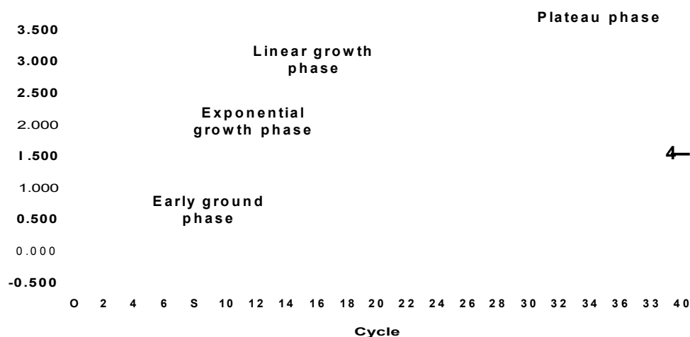
Fig 2.2. Real time PCR amplification curve showing the four major phases.
