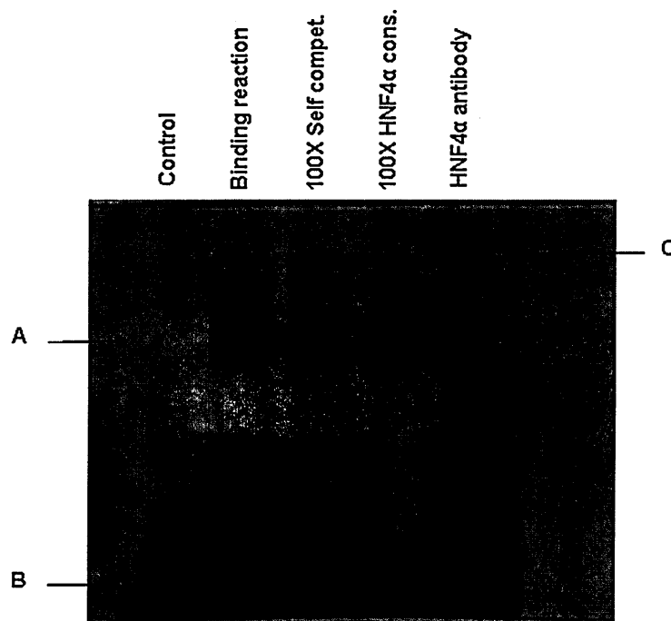
Fig 4.4. Supershift assay using the pZHNH4 \alpha -fluorescent (cy5.5) binding site. Control is the pHNF4 \alpha probe (-48/-38) without HepG2 NE. Binding reaction was the pZHNH4 \alpha probe (-48/-38) with HepG2 NE. Self competitor is the pZHNH4 \alpha probe, the HepG2 NE and the unlabeled pZHNH4 \alpha . HNF4 \alpha consensus lane is the pZHNH4 \alpha probe, the HepG2 NE and unlabeled HNF4 \alpha binding consensus. HNF4 \alpha antibody lane contained the pZHNH4 \alpha probe, the Hep NE and the HNF4 \alpha antibody. Bands indicated by arrow A represent protein DNA complexes. Bands indicated by arrow B represent unbound fluorescent probe. Band C represent the potential antibody-protein-DNA complex. Competition is seen with 100-fold molar excess of self-competitor and the HNF4 \alpha consensus sequences.
