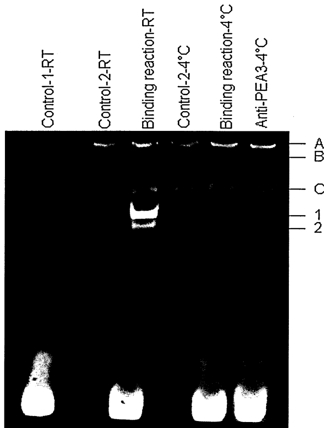
Fig 3.12. Supershift assay at 4°C using biotinylated pPZ ASE binding sites. Control-1 is the pPZ ASE probe without HepG2 NE. Control-2 is the HepG2 NE without probe. Binding reaction is the probe with HepG2 NE. Anti-PEA3 is an antibody against PEA3 protein together with the binding reaction. From left to right, the first three lanes were performed at room temperature (RT) while the other following three lanes were performed at 4°C. Control-2-4°C is the HepG2 NE incubated with the binding buffer overnight at 4°C. Binding reaction-4°C is the HepG2 NE incubated with the binding buffer overnight at 4°C followed by incubation with the probe for 30 minutes at room temperature. Anti-PEA3-4°C is the antibody incubated with the HepG2 NE overnight at 4°C and further incubated with the probe for 30 minutes at room temperature. No supershift was seen. A, B and C are control bands which come up whenever the HepG2 NE is added. Bands 1 and 2 are the protein-DNA complexes. Protease inhibitor cocktail and the DTT were added to the binding buffer just before the assay.
