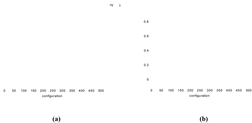
Figure 5.29: LZ=8K_1(\theta_0) : Components of the director in the a)homeotropic region and b)planar region .
