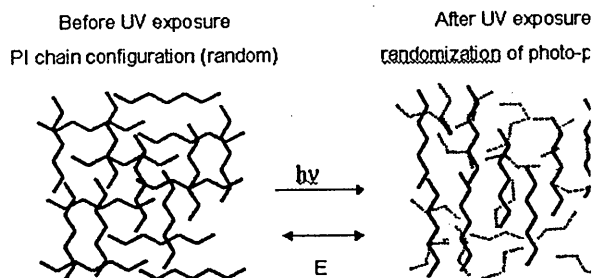
Figure 2.20: Schematic mechanism of polyimide degradation.
