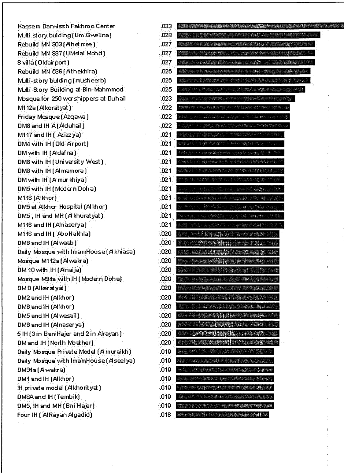
Figure 4.14. Priority selection
