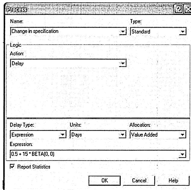
Figure 6.11 Process Entity
