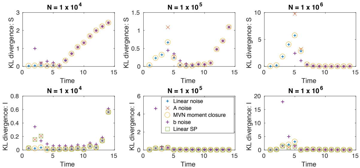
Figure 3: Numerical comparisons of the approximation schemes with stochastic simulations of the SIR model using the KL divergence. Within each subplot (a-c) different rate constant parameter values were used to generate stochastic simulations for comparison to each Gaussian approximation. The size of the susceptible population is compared on the top line and the size of the infectious population on the bottom line, for three population sizes (increasing from left to right).
