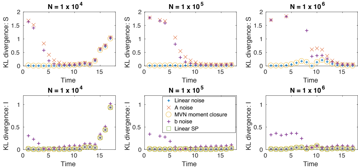
(c) \beta = 3, \gamma = 0.5 ( R_0 = 6 )
