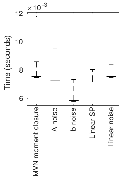
Figure 4: Running time for the sets of ordinary differential equations for each of the approximation methods with \beta = 2 , \gamma = 1 , and N = 1 \times 10^6 . (The box denotes the median, lower quartile, and upper quartile. Whiskers extend to the maximum and minimum. When the interquartile range is narrow, as here, the box displays as simply a thick line.)
