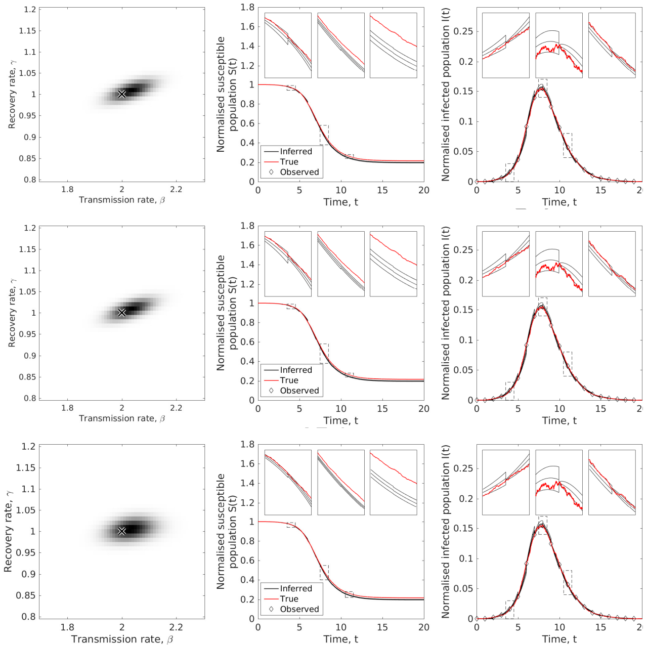
Figure 5: Inference of the susceptible population using the multivariate normal moment closure (top), linear noise (middle), and A noise (bottom) Gaussian process approximations. Left: likelihood (density plot) is concentrated around the true value (cross). Centre: Data on the number of infecteds allows for good reconstruction of the unobserved susceptibility over time. Shown are the synthetic data ('True', red), the mean of the approximation scheme using the inferred parameter values ('Inferred', black), and the mean plus/minus one standard deviation (black) in both the main figures and insets. Dashed rectangles on the main figures show the locations of the insets from left to right. Right: Data ('Observed', diamonds) allow for good reconstruction of the number of infecteds over time. The red lines, black lines, and dashed rectangles are as before.
