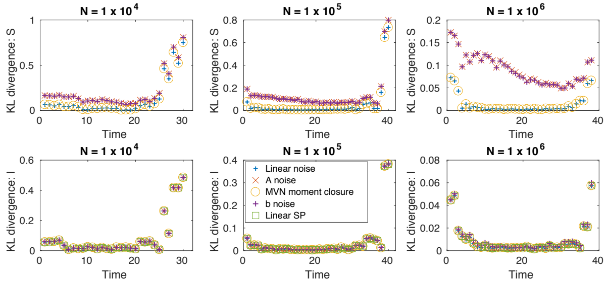
(b) \beta = 2, \gamma = 1 ( R_0 = 2 )
