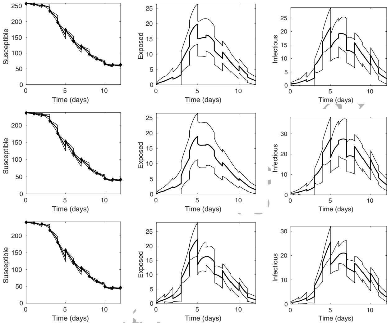
Figure 6: Inference of the susceptible (left), exposed (centre), and infectious (right) population using the multivariate normal moment closure approximation (top), the linear noise approximation (middle), and the A noise approximation (bottom) from data of the number of new cases of norovirus per day on a cruise ship. The black diamonds (left) are our known values which we obtain from the data reported by Vivancos et al. (2010), as described in the text. The dark lines are the mean and light lines are the mean plus/minus one standard deviation.
