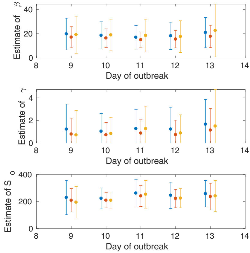
Figure 7: Estimates of the model parameters \beta , \gamma , and S_0 as the epidemic progresses for the multi-variate normal moment closure approximation (blue), the linear noise approximation (red), and the A noise approximation (yellow). The dots are maximum likelihood estimates and the bars give 95% confidence intervals.
