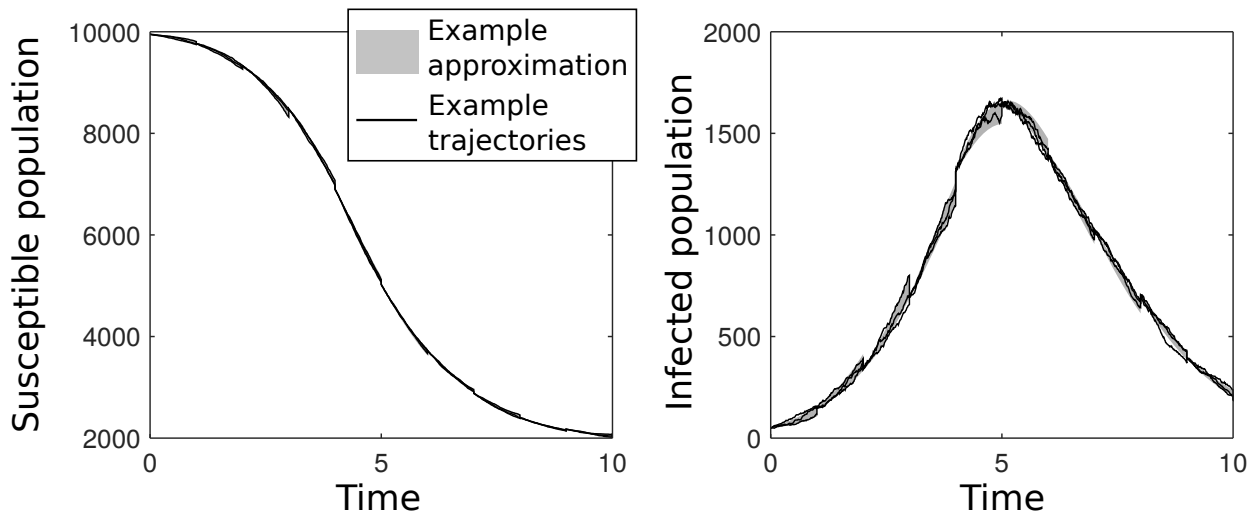
Figure 2: A typical example of stochastic trajectories and one Gaussian process approximation. This example was generated with parameters \beta = 2 , \gamma = 1 , and N = 1 \times 10^4 and the multivariate normal moment closure approximation. The shaded approximation region corresponds to the mean plus/minus one standard deviation.
