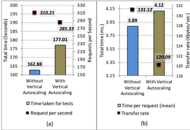
Fig. 18. Comparison between total time of tests, requests per second, time per request and transfer rate for the two cases of vertical and non-vertical autoscaling
