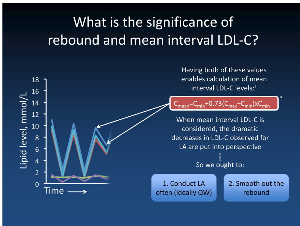
Figure 5 Rebound and calculated mean interval LDL-C govern LA frequency. Mean interval LDL-C calculation 55 based on representative patient case; *Coefficient of 0.64 is also used. LA, lipoprotein apheresis; LDL-C, low-density lipoprotein cholesterol; QW, once weekly.
