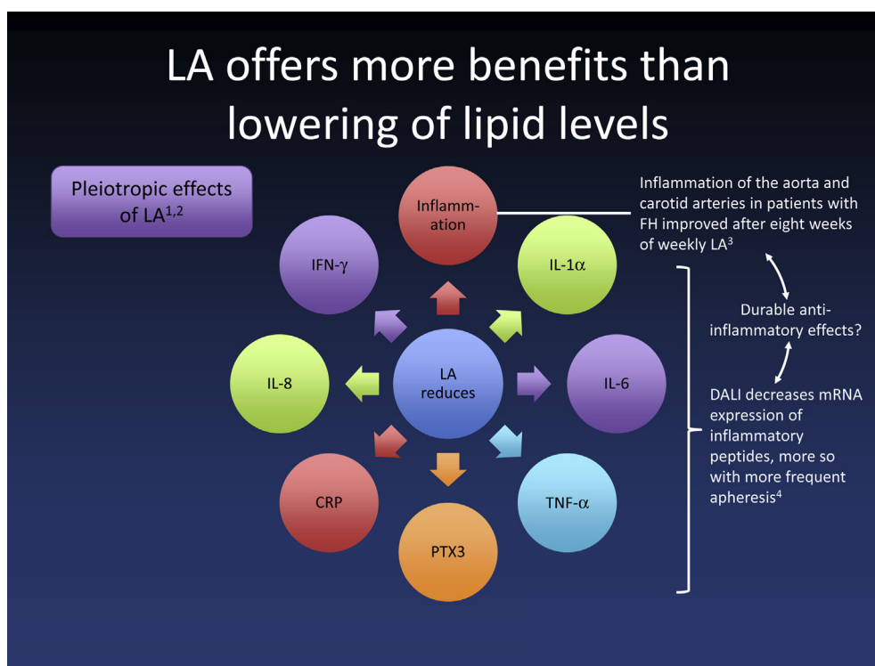
Figure 2 Lipoprotein apheresis offers more benefits than lowering of lipid levels. Pleiotropic effects of lipoprotein apheresis (LA). 31–33 LA reduces the expression and/or activity of a range of immunocompetent cytokines. CRP, C-reactive protein; DALI, direct adsorption of lipids; IFN, interferon- \gamma ; IL- \alpha , interleukin- \alpha ; PTX3, pentraxin-3; TNF- \alpha , tumor necrosis factor- \alpha .
