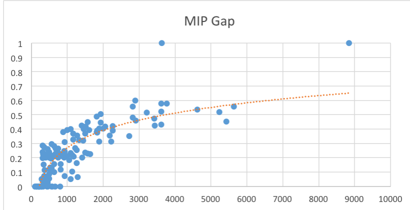
Figure 2: Optimality gap versus instance size (the number of variables in the problem formulation of Section 2) for ILPG.
