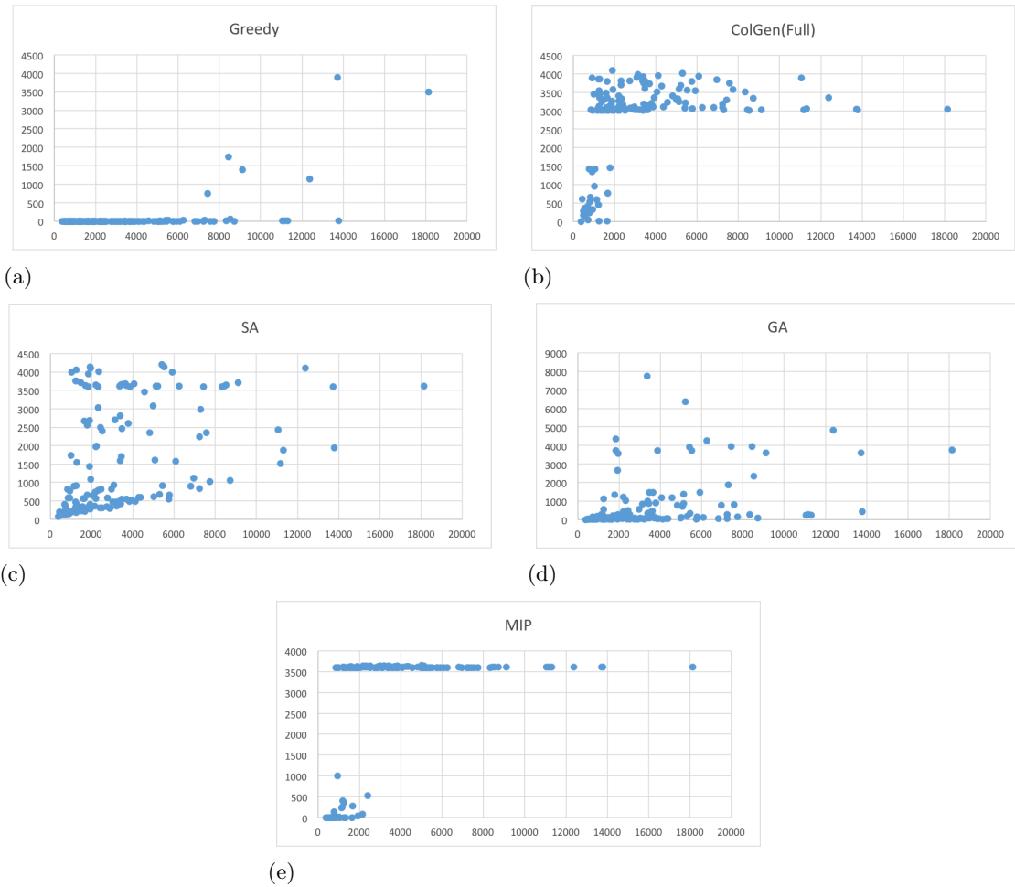
Figure 1: Average computation time versus instance size (the number of variables in the problem formulation of Section 2) for (a) GR, (b) CGG, (c) SA, (d) GA, and (e) ILPG.
