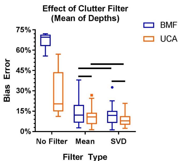
Fig. 4. Effect of clutter filter on the resultant ePIV bias. Using a clutter filter significantly improves accuracy for both BMF and UCA. n=9 . *solid lines denote p>0.05 (no significance)
