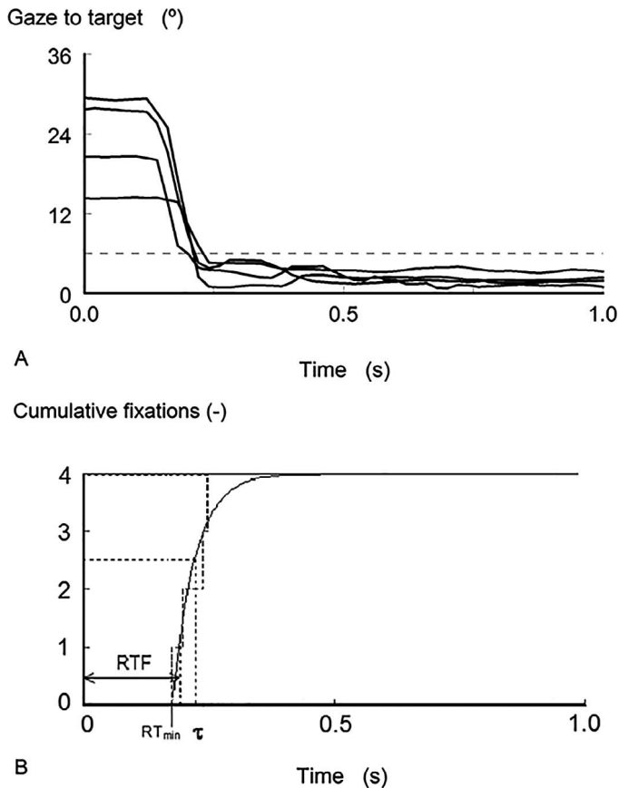
Figure 3. Panel A shows four gaze responses of one subject expressed as the distance from the center of the target area (degrees of visual angle, y -axis), over time (seconds, x -axis). In panel B, the corresponding reaction times of these responses are arranged in a cumulative plot. An exponential curve was fitted to this plot to quantify this subject's reaction time to fixation (RTF): the sum of the minimum reaction time ( RT_{min} ), and 1/3 of the time constant \tau of the exponential curve.
