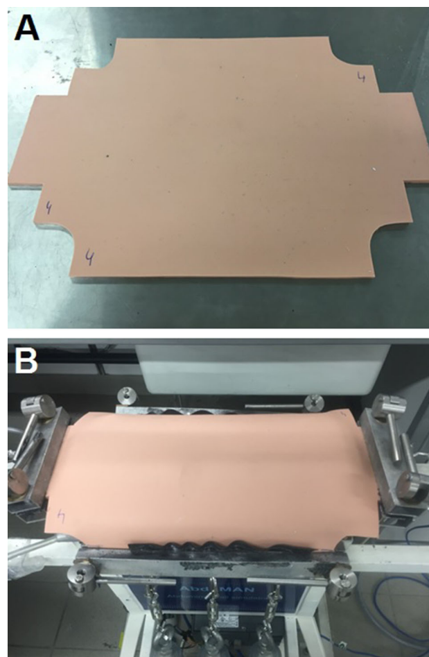
Fig. 2 Abdominal wall samples. a Shape of a sample prior to mounting. b A mounted sample on the 'AbdoMAN' device with fixation in four directions
