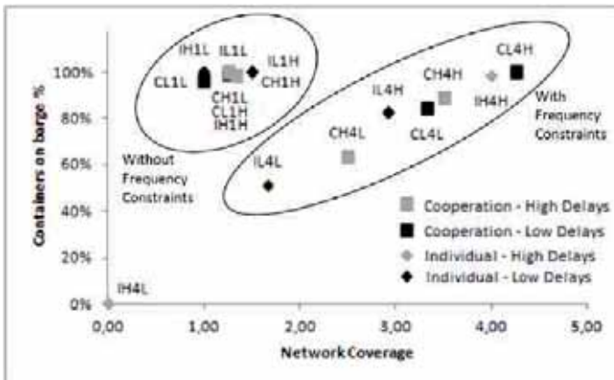
Figure 5.6: Network Coverage vs Containers on barge
