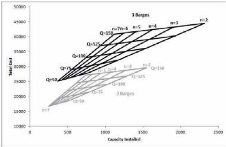
Figure 5.11: Capacity installed vs Total cost
