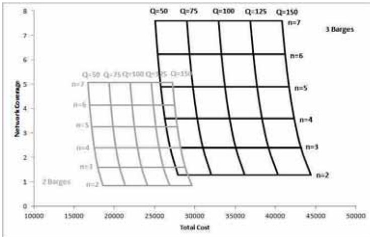
Figure 5.12: Network coverage vs Total costs
