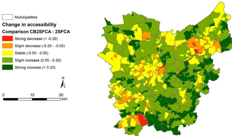
Fig. 10. Accessibility to daycare centers in East Flanders by implementing the 2SFCA and CB2SFCA methods
