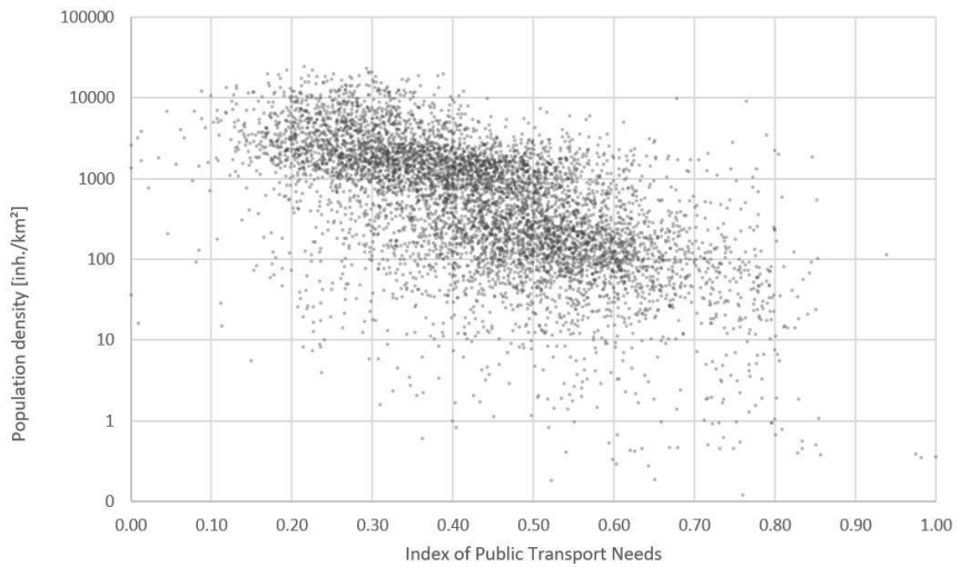
Fig. 16. The Index of Public Transport Needs in relation to the population density per TAZ
