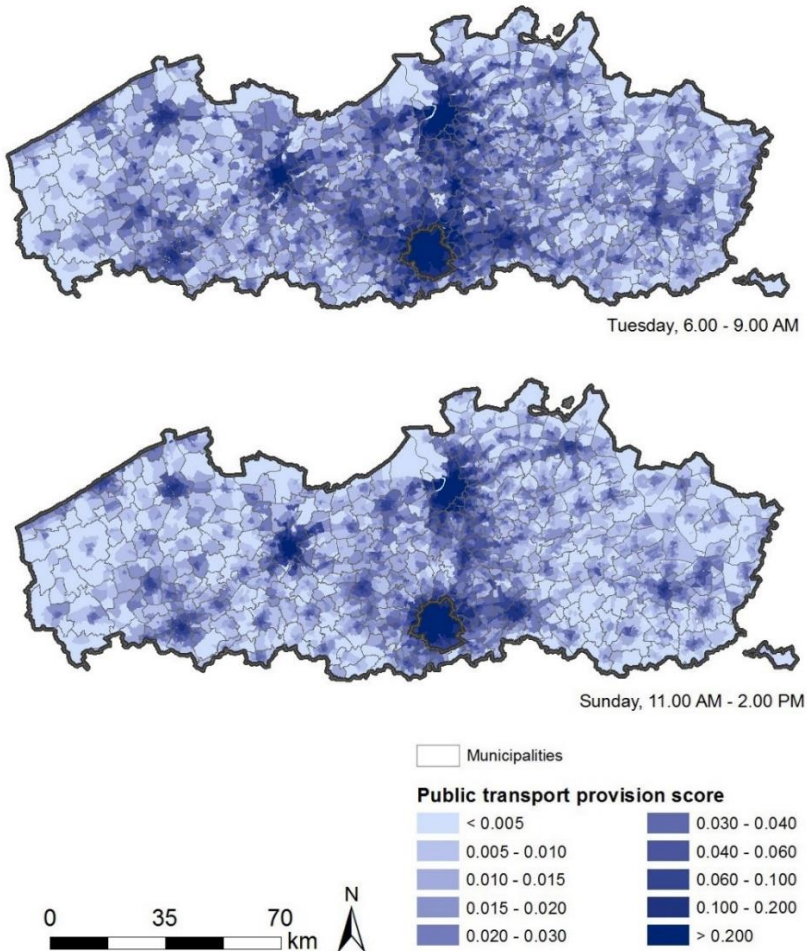
Fig. 18. Public transport provision indices per TAZ for Flanders and Brussels, for various times of the week
